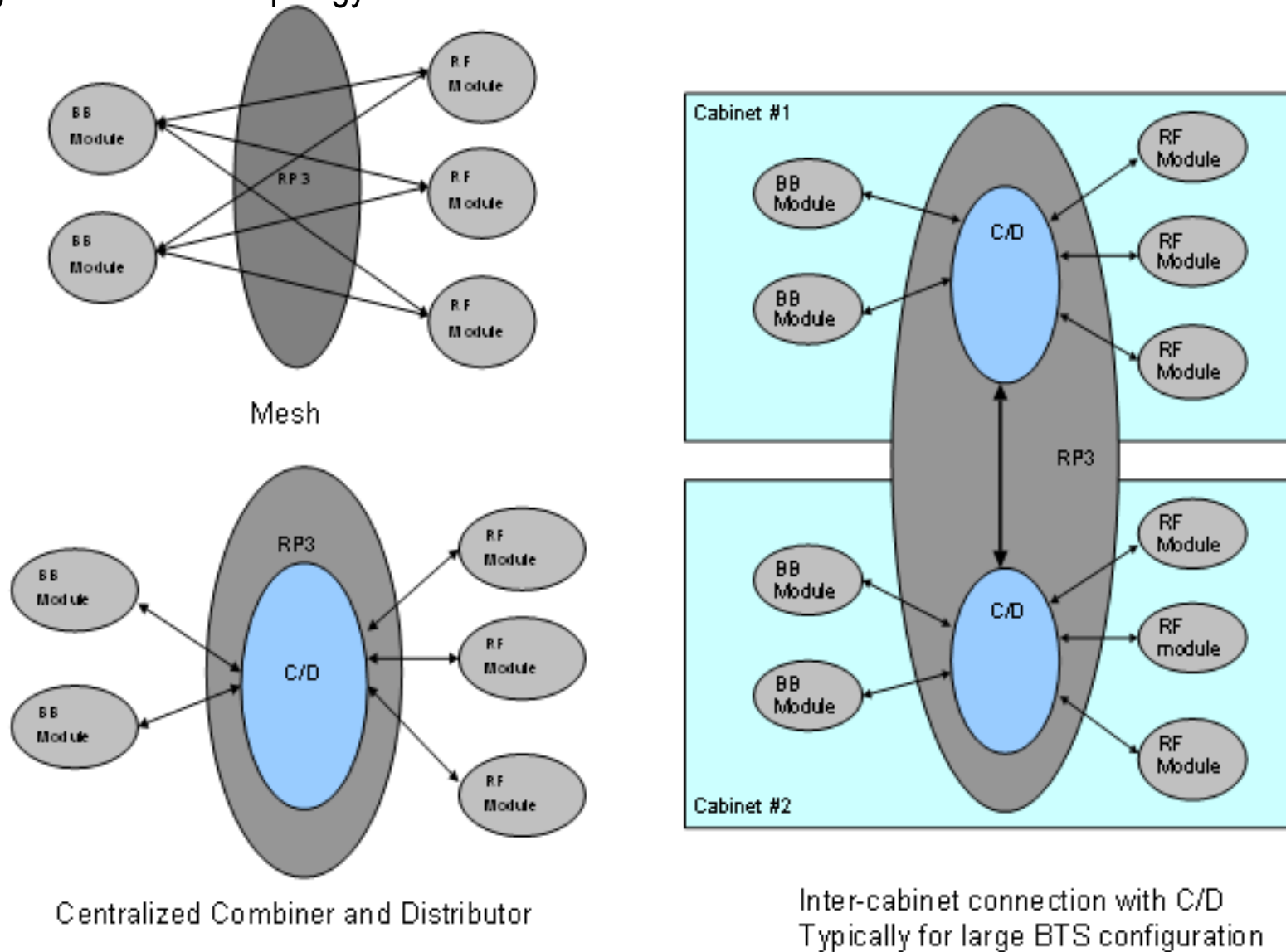
Figure 2: BTS RP3 topology
