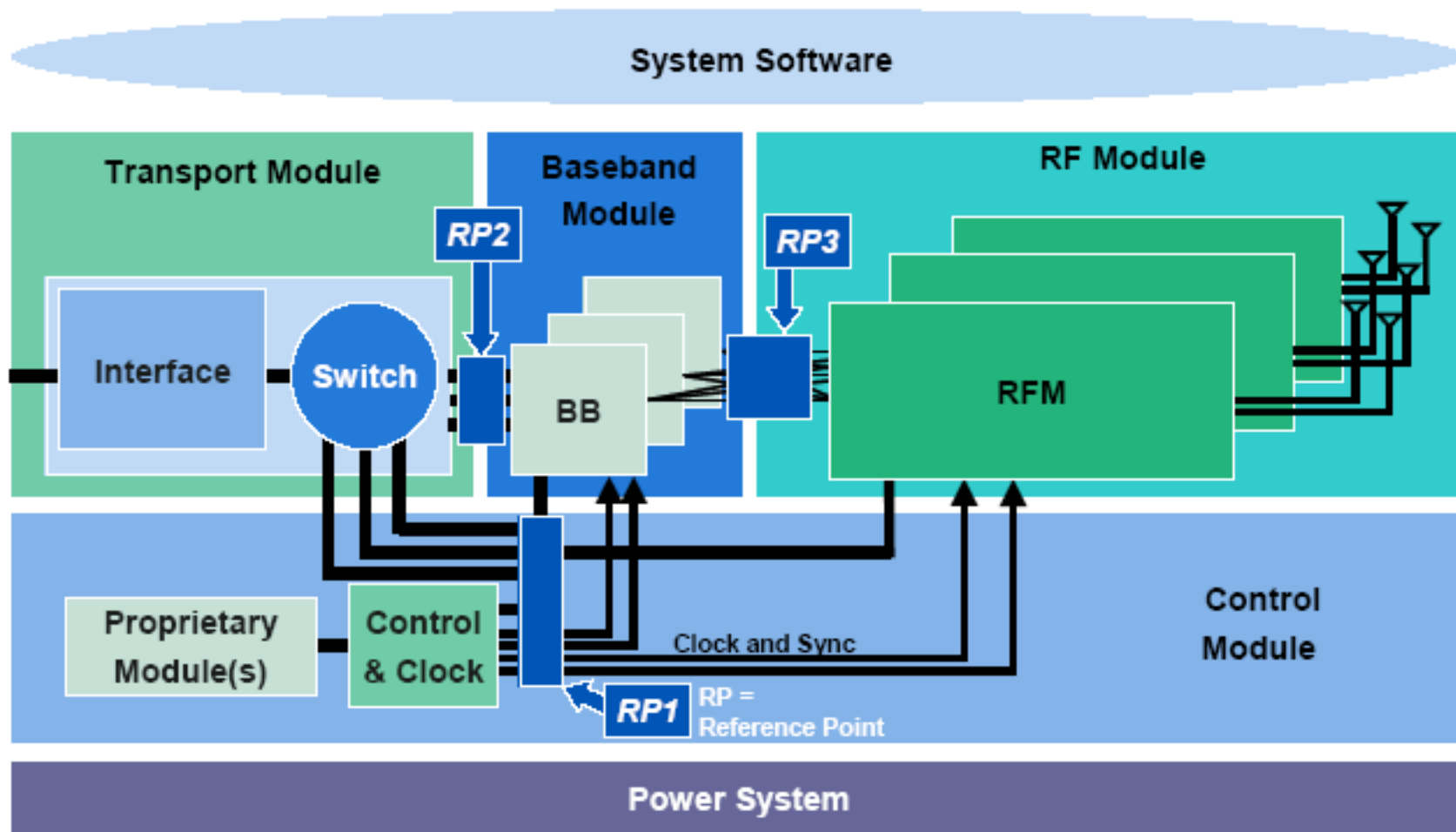
Figure 1. Base Station Overview
