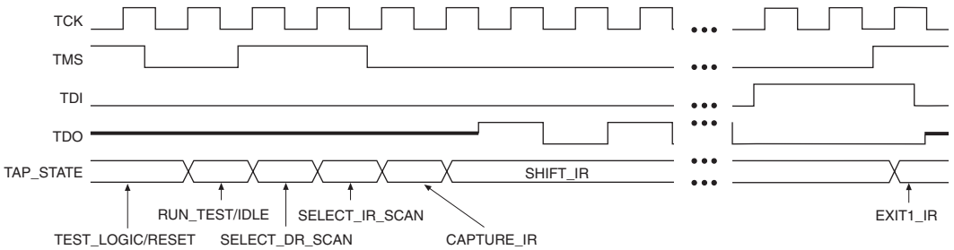
Figure 12. Selecting the Instruction Mode
