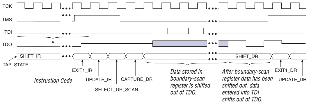
Figure 16. EXTEST Shift Data Register Waveforms
