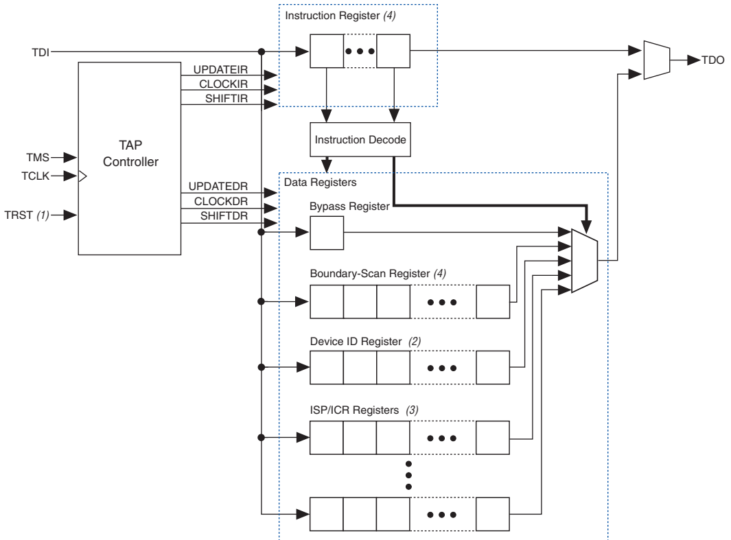
Figure 2. IEEE Std. 1149.1 Circuitry
