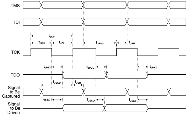
Figure 11. IEEE Std. 1149.1 Timing Waveforms
