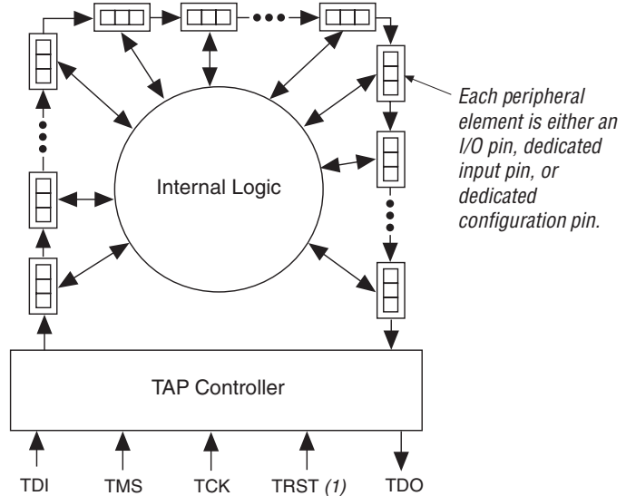
Figure 3. Boundary-Scan Register
