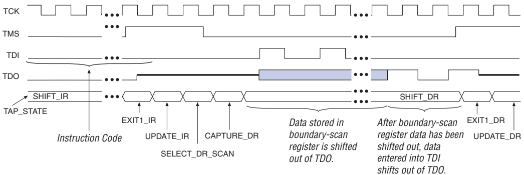
Figure 14. SAMPLE/PRELOAD Shift Data Register Waveforms
