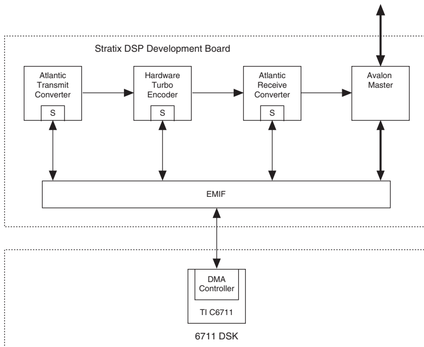
Figure 1. Block Diagram Note (1)
