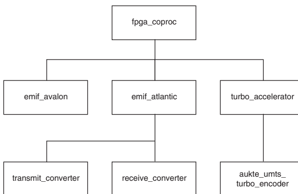
Figure 5. Module Heirarchy
