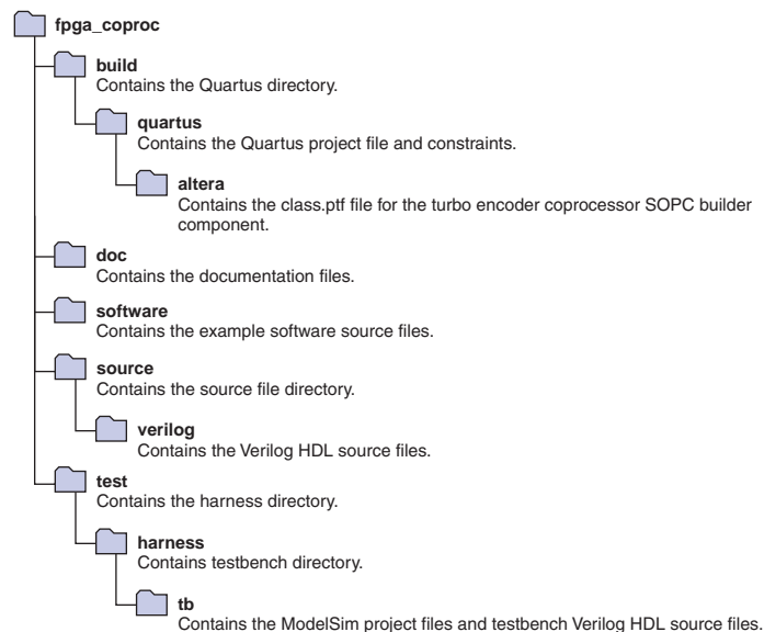
Figure 4. Directory Structure
