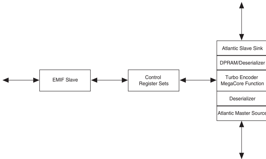
Figure 3. Hardware Turbo Encoder
