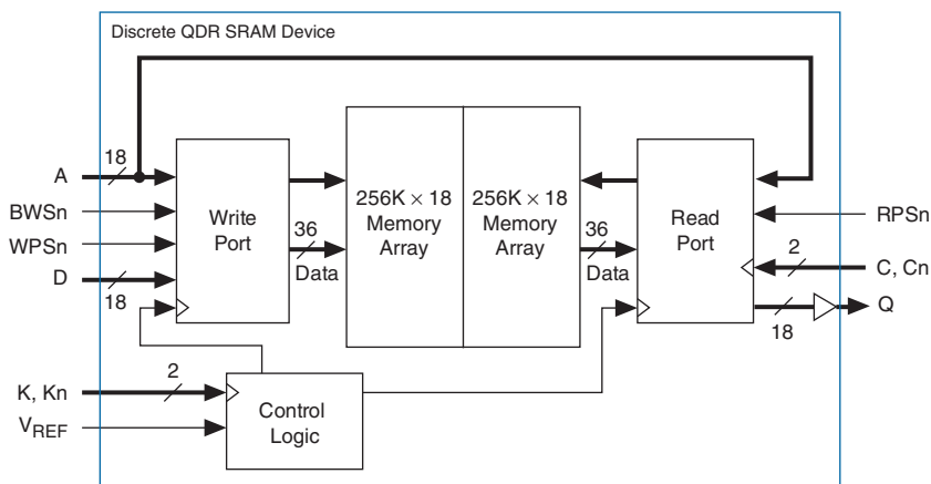
Figure 2. QDR SRAM Burst-of-2 Architecture
