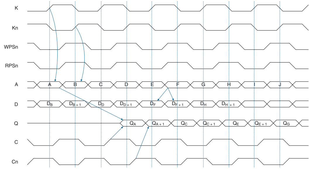
Figure 3. Burst-of-2 Timing Diagram
