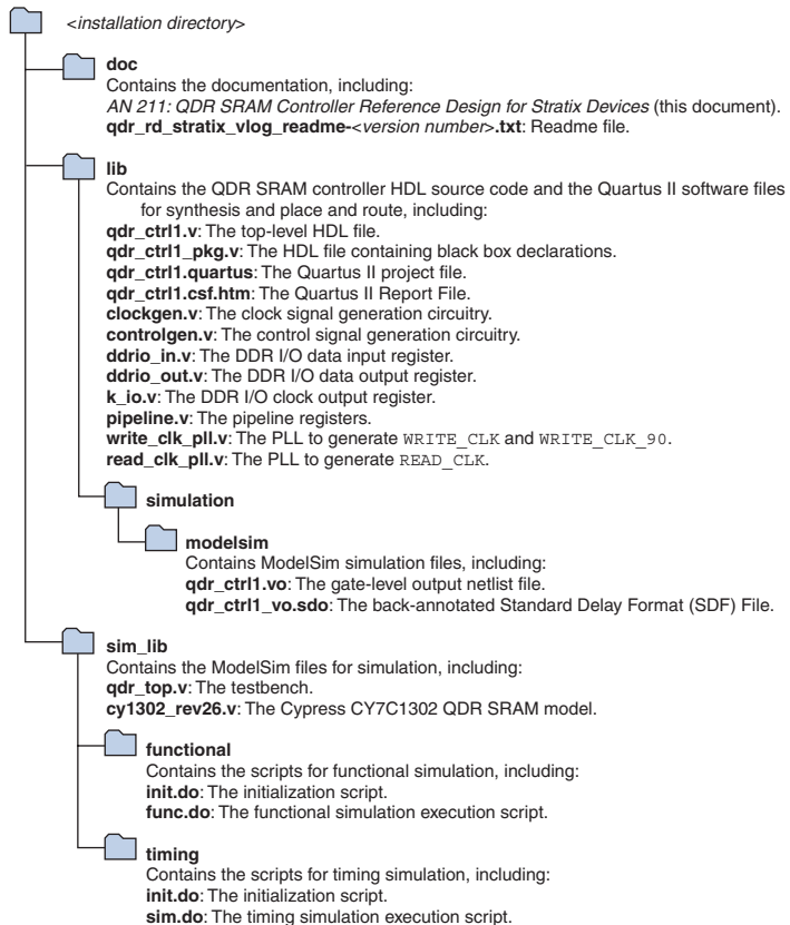
Figure 12. QDR SRAM Controller Directory Structure
