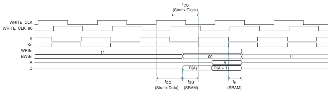
Figure 10. Write Cycle Timing Waveform
