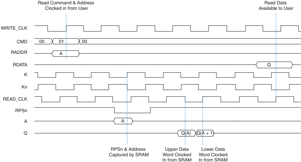
Figure 7. Read Cycle Waveform (Burst-of-2)
