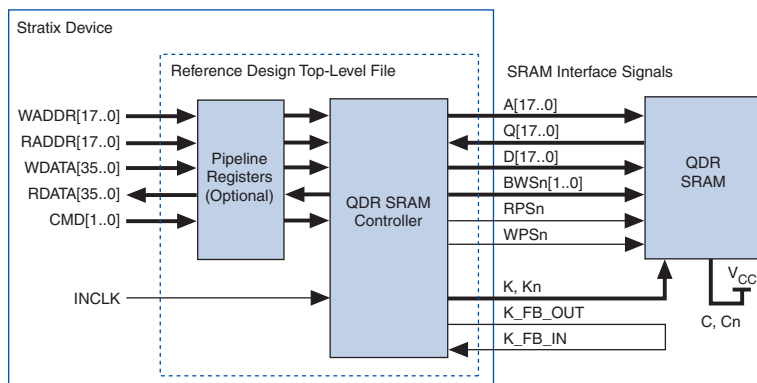
Figure 5. QDR SRAM Controller Reference Design Block Diagram
