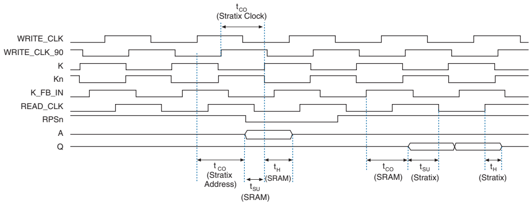
Figure 11. Read Cycle Timing Waveform
