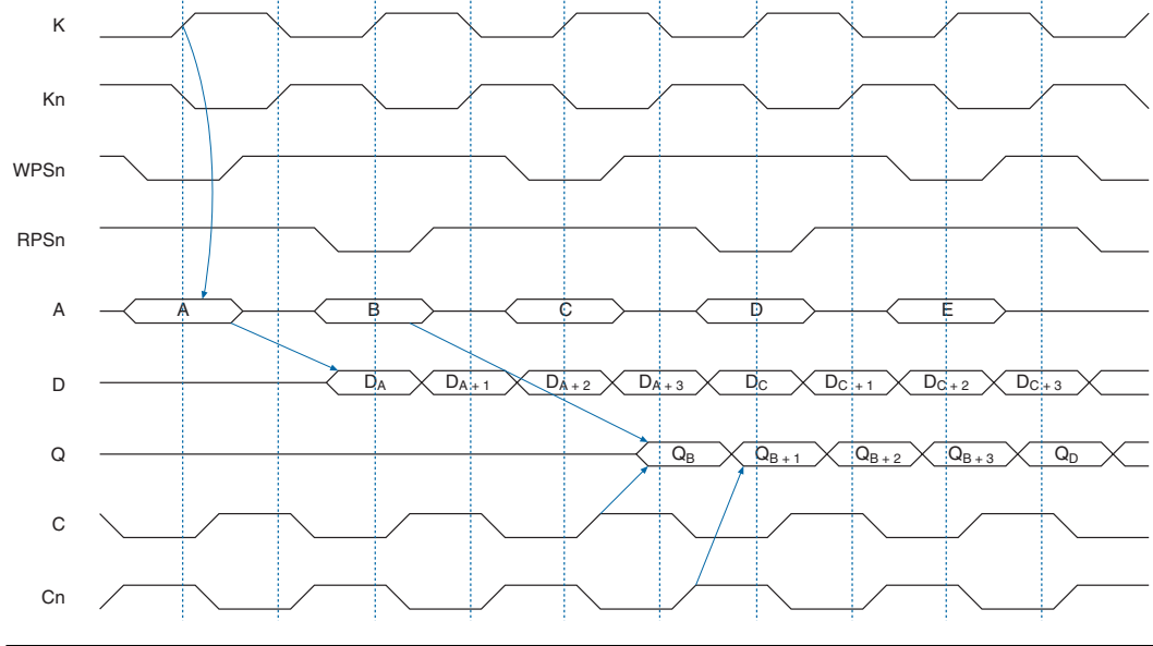
Figure 4. Burst-of-4 Timing Diagram
