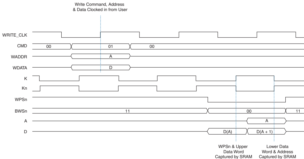
Figure 6. Write Cycle Waveform (Burst-of-2)
