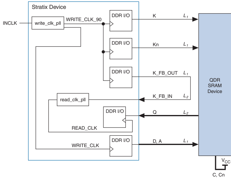
Figure 9. Clock Generation Note (1)
