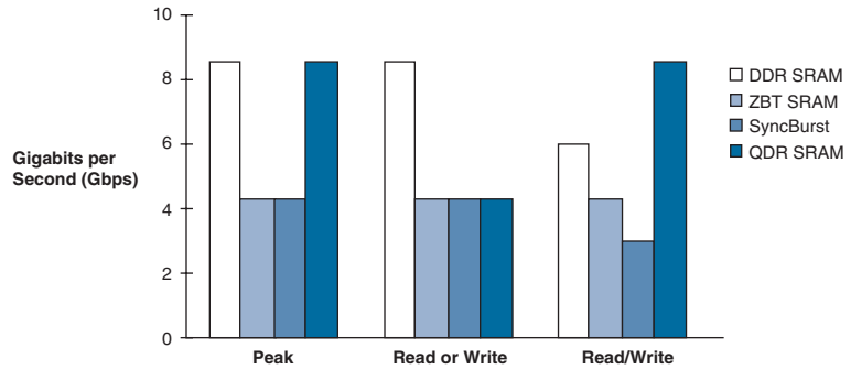
Figure 1. SRAM Memory Architecture Performance Comparison Note (1)
