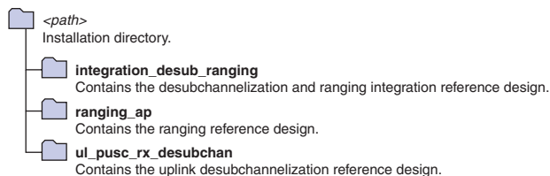
Figure 3. Directory Structure
