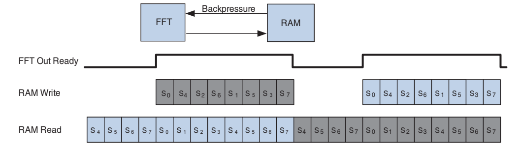
Figure 4. A Memory Efficient Implementation of Cyclic Prefix Insertion with Backpressure
