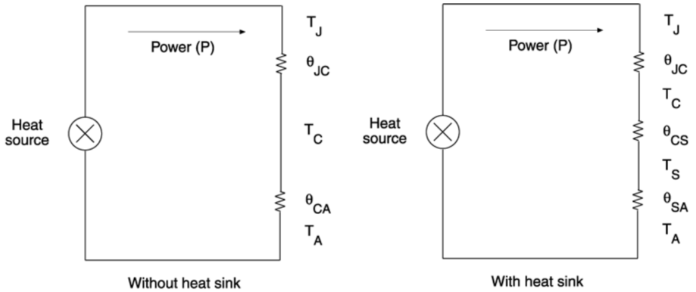
Figure 1. Thermal Circuit
