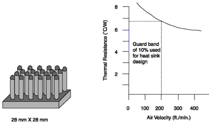
Figure 2. Heat Sink & Thermal Resistance Curve for Example Application Requiring a Heat Sink
