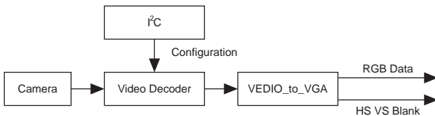
Figure 8. Video Decoding Schematic Diagram
