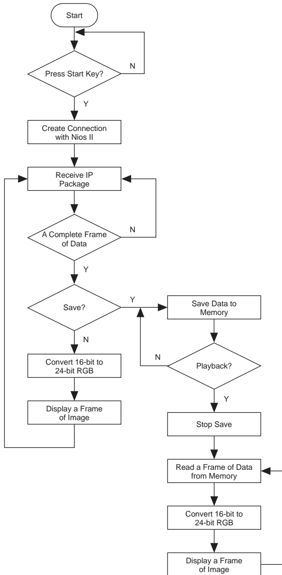
Figure 18. Client Application Flow Chart
