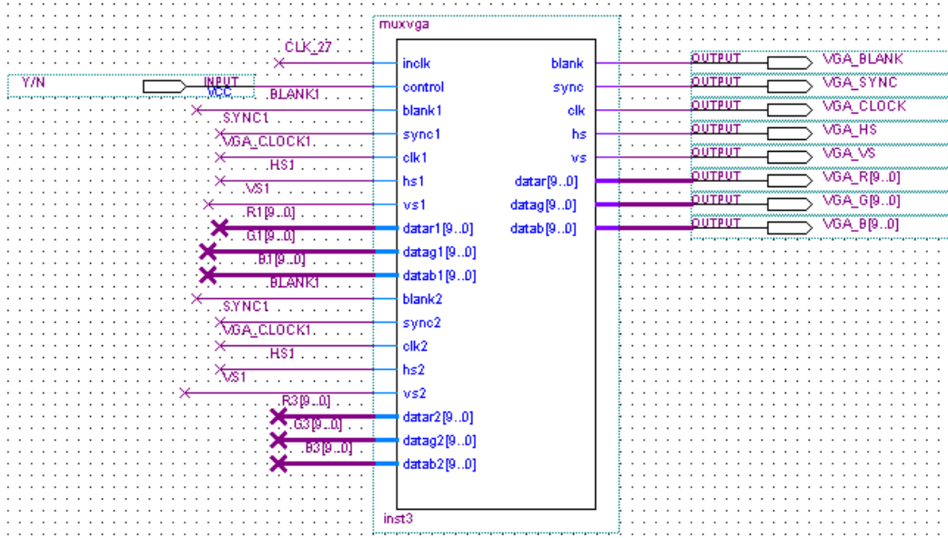
Figure 16. VGA Display Selection Module Schematic Diagram
