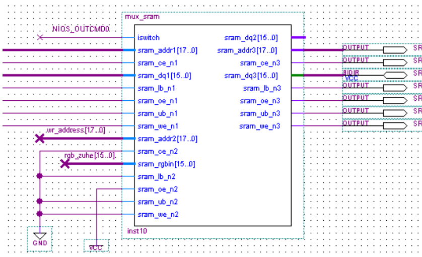
Figure 14. SRAM Bus Switching Module Schematic Diagram
