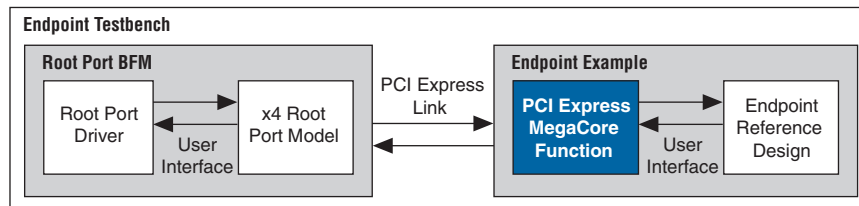
Figure 1. Endpoint Testbench
