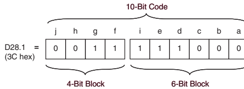
Figure 4–2. 10-Bit Grouping of 6-bit &amp; 4-Bit Sub-Blocks
