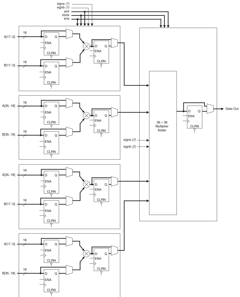
Figure 10–9. 36-Bit Multiplier
