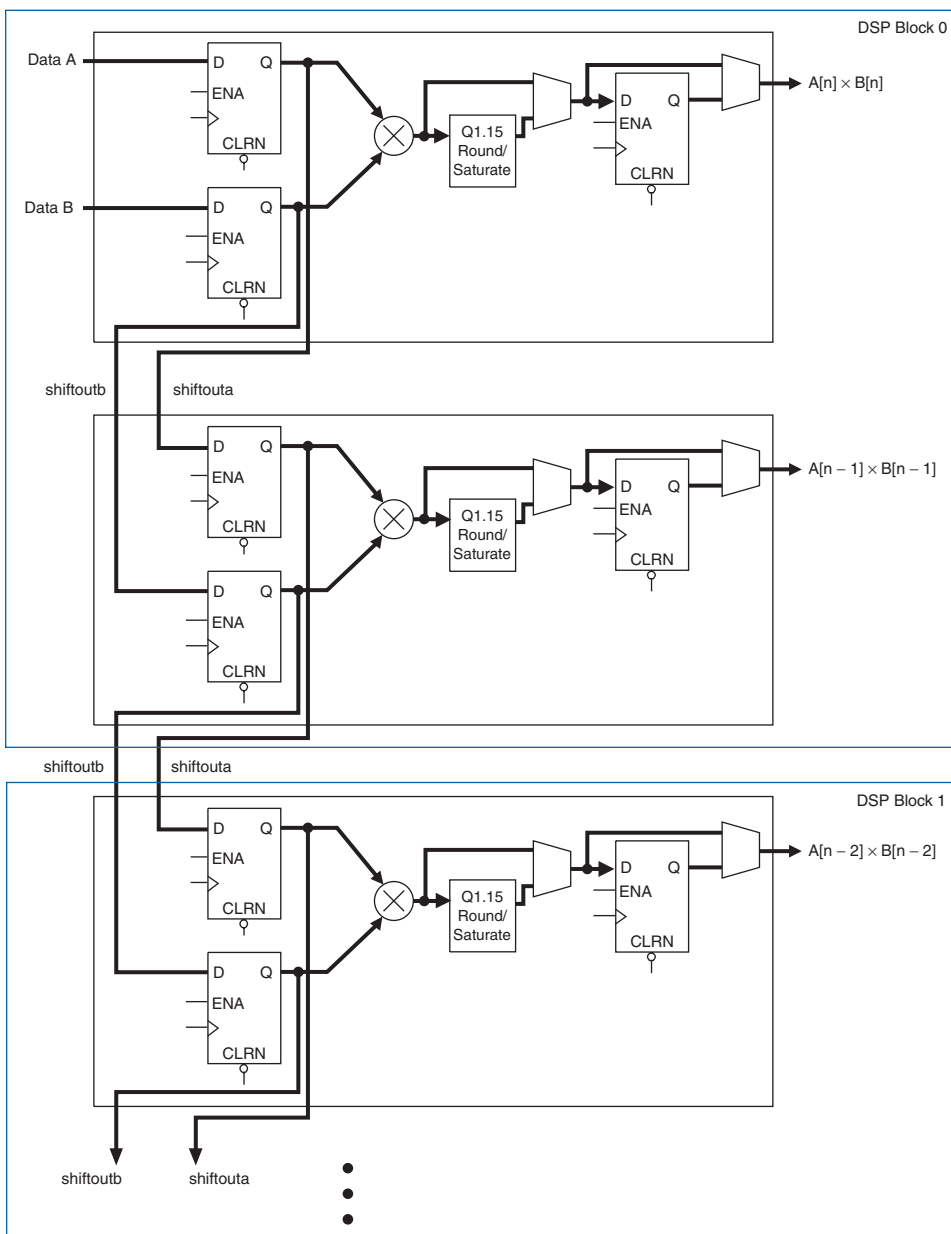
Figure 6-5. Shift Register Chain Note (1)
