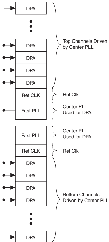
Figure 10–20. Driving Capabilities of a Center Fast PLL
