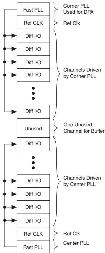
Figure 10-21. Usage of Corner & Center Fast PLLs Driving DPA Channels in a Single Bank
