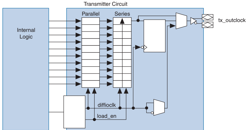
Figure 10–4. Transmitter in Clock Output Mode
