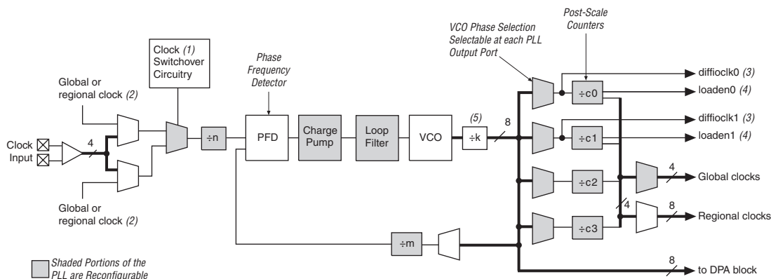
Figure 10–11. Fast PLL Block Diagram
