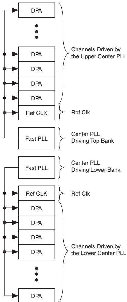
Figure 10–22. Center Fast PLL Usage When Driving DPA Channels
