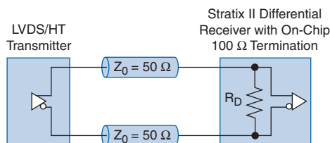
Figure 10–10. On-Chip Differential Termination
