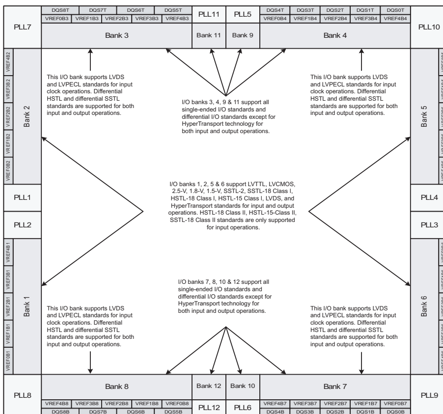
Figure 10–1. Stratix II I/O Banks Note (1), (2), (3), (4), (5), (6), and (7)
