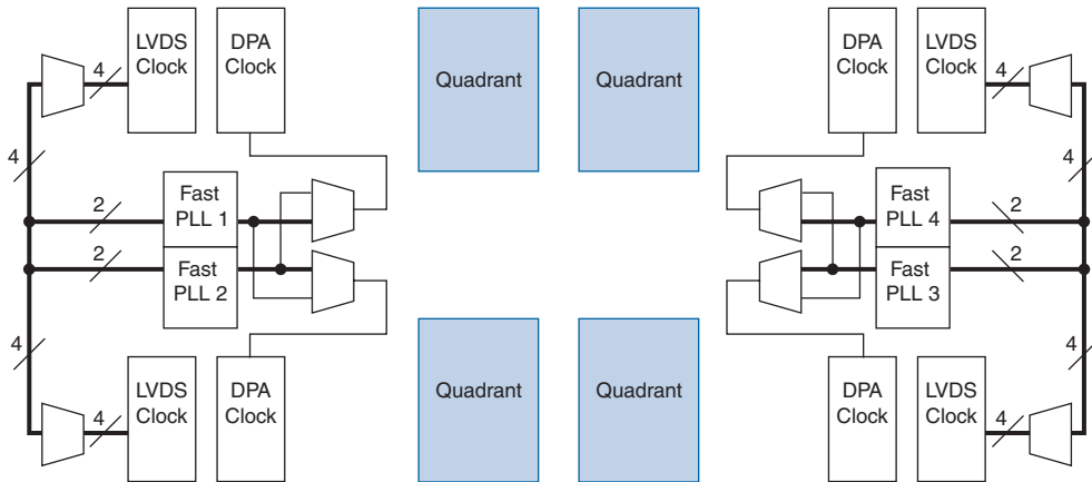
Figure 10–12. Fast PLL & LVDS/DPA Clock for EP2S15, EP2S30, and EP2S60 Devices Note (1)
