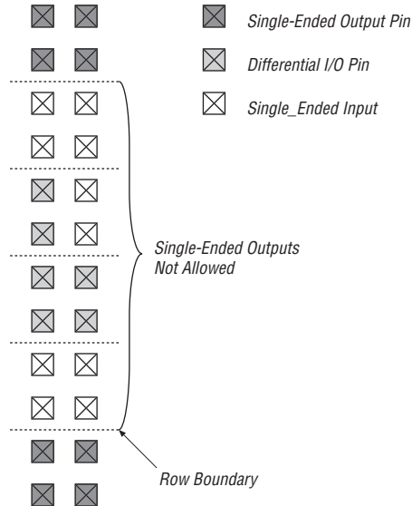
Figure 10–19. Single-Ended Output Pin Placement with Respect to Differential I/O Pins
