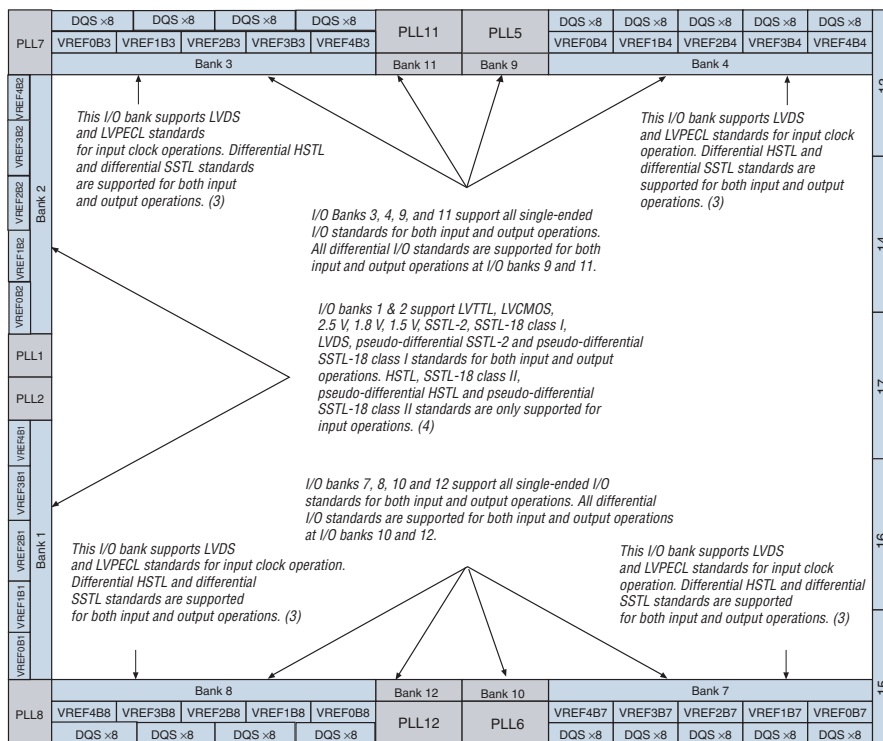
Figure 10–2. Stratix II GX I/O Banks Note (1), (2), (3), (4), (5), (6), and (7)
