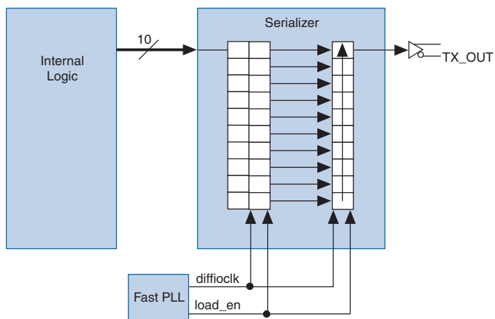
Figure 10–3. Transmitter Block Diagram
