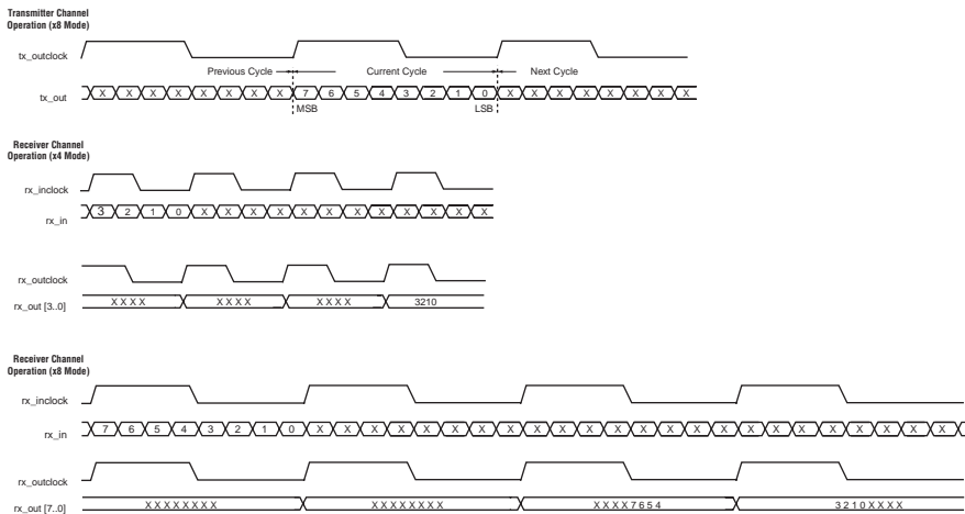
Figure 10–17. Bit Order for One Channel of Differential Data
