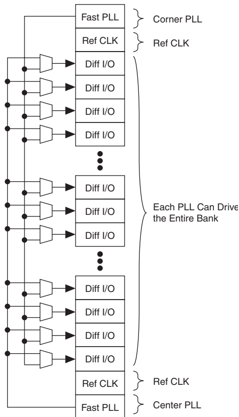
Figure 10–23. Fast PLL Driving Capability When Driving Non-DPA Differential Channels
