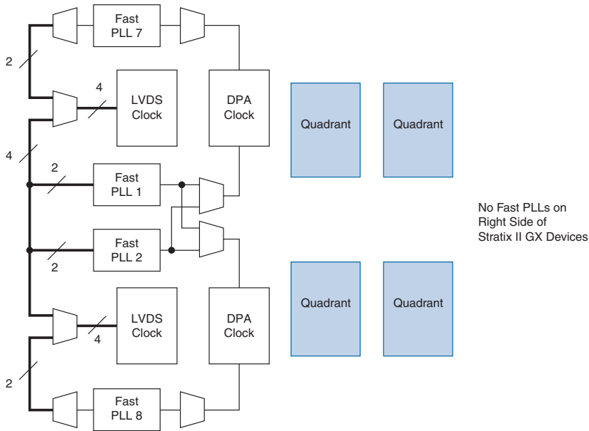
Figure 10-15. Fast PLL & LVDS/DPA Clocks for EP2SGX60E, EP2SGX90 & EP2SGX130 Devices
