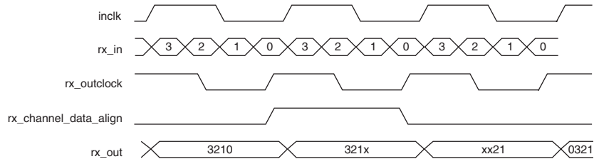
Figure 10–8. Data Realignment Timing
