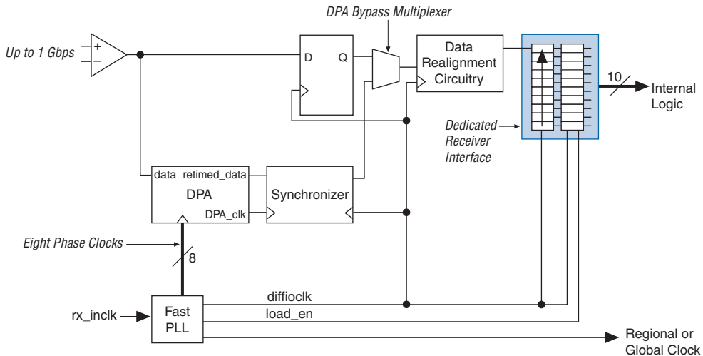
Figure 10–6. Receiver Block Diagram
