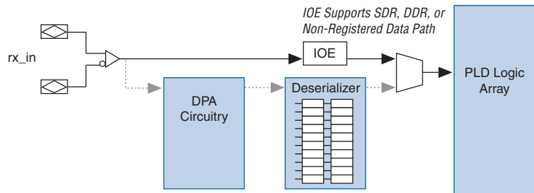
Figure 10–7. Deserializer Bypass
