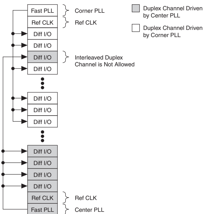
Figure 10–24. Illegal Placement of Interlaced Duplex Channels in an I/O Bank
