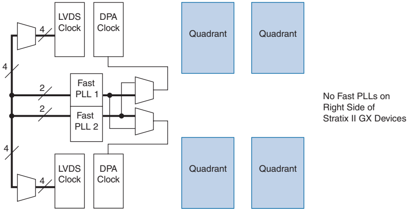
Figure 10-14. Fast PLL & LVDS/DPA Clock for EP2SGX30C/D & EP2SGX60C/D Devices
