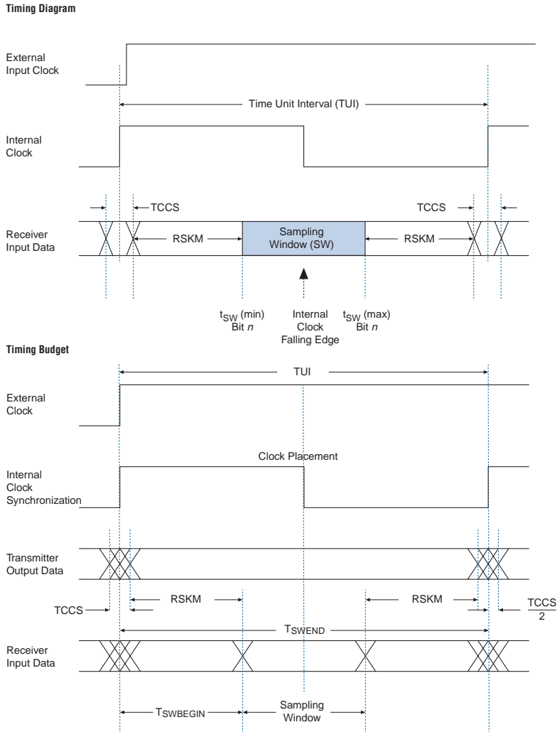
Figure 10–18. Differential High-Speed Timing Diagram & Timing Budget for Non-DPA
