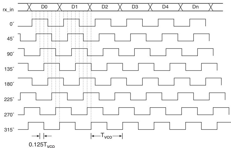
Figure 10–9. DPA Clock Phase to Data Bit Relationship
