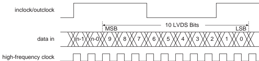
Figure 10–16. Bit Orientation in the Quartus II Software
