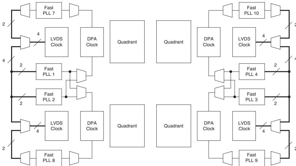
Figure 10–13. Fast PLL & LVDS/DPA Clocks for EP2S60, EP2S90, EP2S130 & EP2S180 Devices Note (1)
