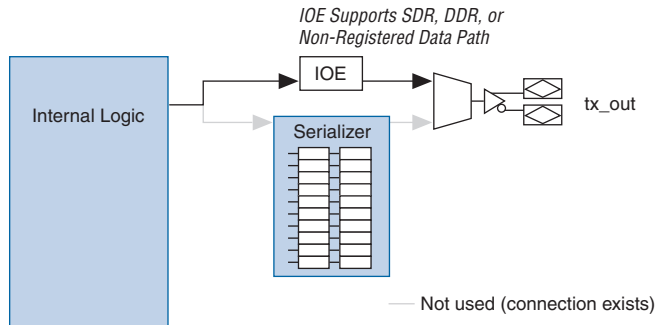
Figure 10–5. Serializer Bypass
