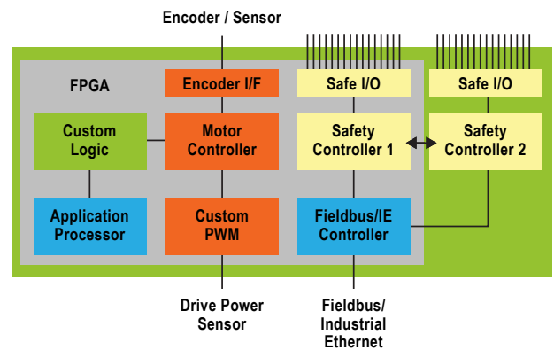
Figure 1: A Typical SIL3 Industrial “Safe” System
