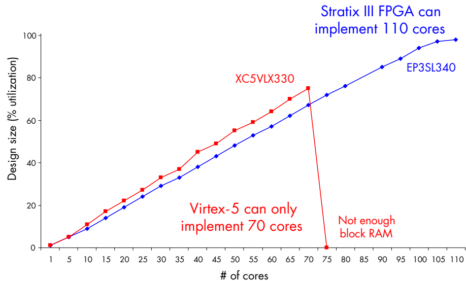
Figure 2. Design size (% utilization) vs. number of cores
