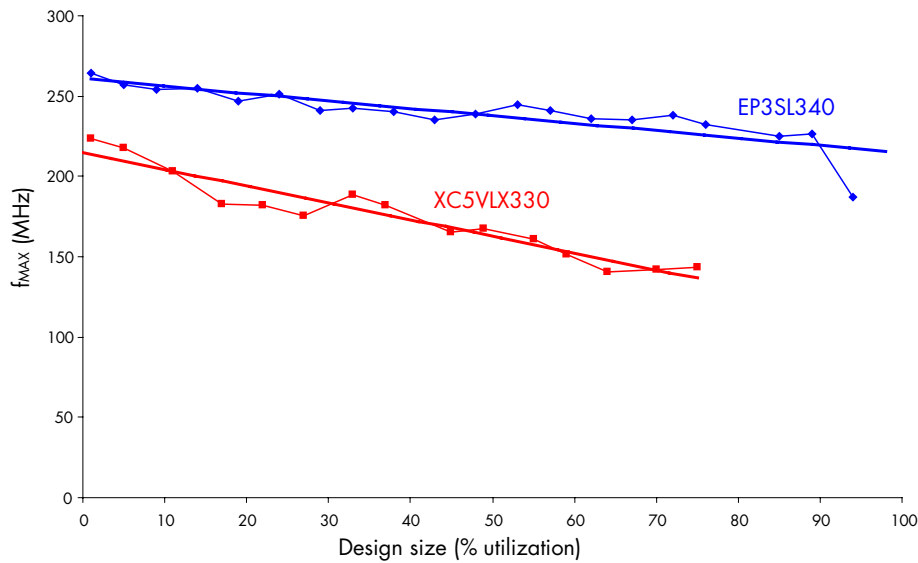
Figure 1. f_{MAX} vs. design size (% utilization)
