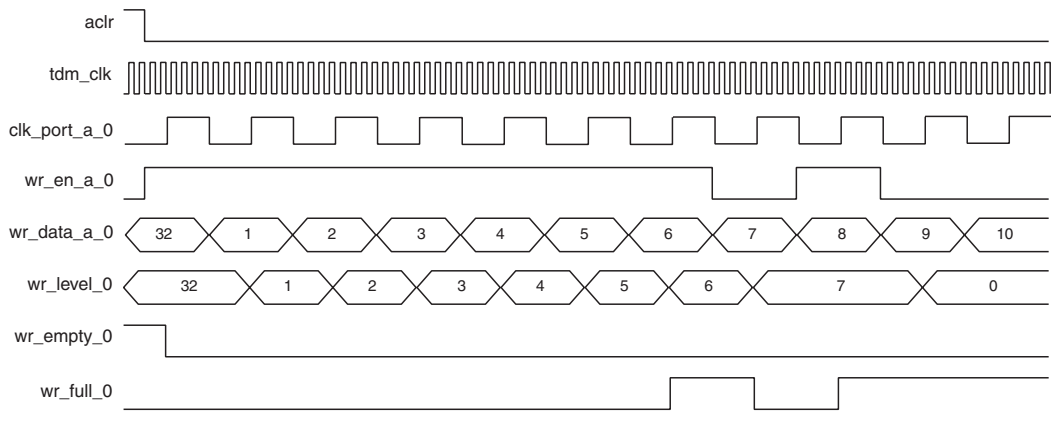
Figure 6. Initializing and Writing to a FIFO
