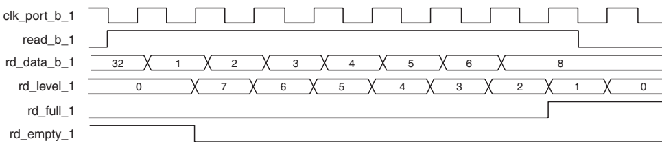
Figure 8. Using read_b_n as a Read Acknowledge
