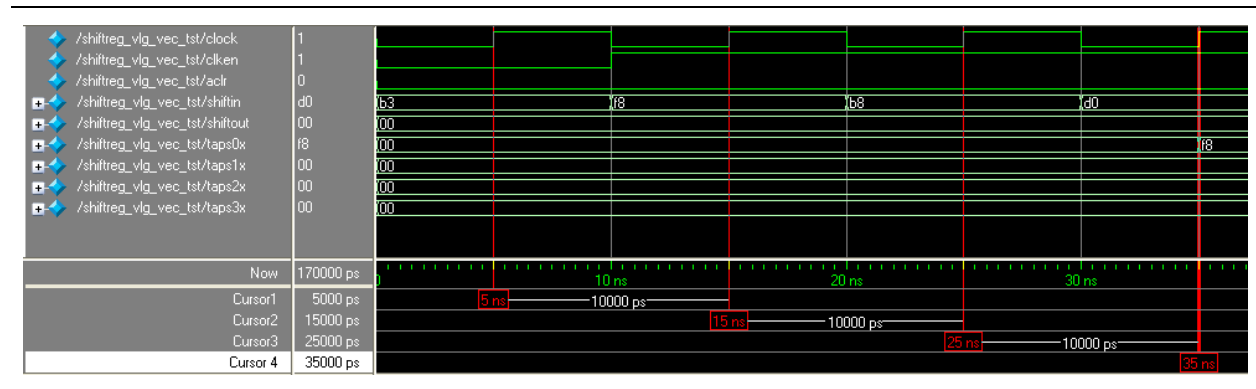
Figure 2-9. First Three Data Written and Shifted in the Shift Register
