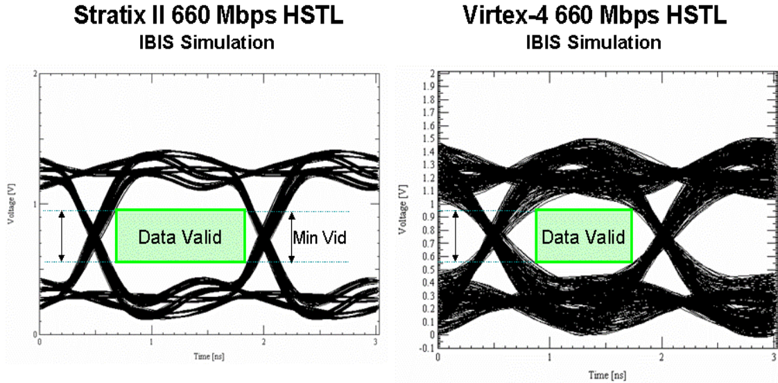
Figure 5: 660 Mbps HSTL IBIS Simulation comparison of Stratix II and Virtex 4 eye-diagrams
