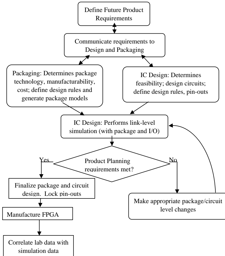
Figure 8: Altera Silicon-Package Co-Design Methodology
