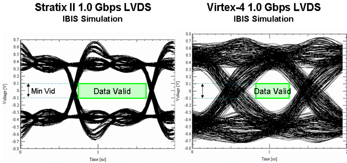
Figure 4: 1.0 Gbps LVDS IBIS Simulation comparison of Stratix II and Virtex 4 eye-diagrams
