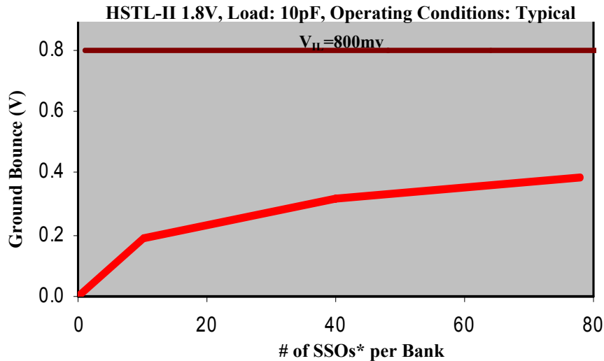
Figure 7: Chart of Stratix II HSTL-II 1.8V I/O SSN Performance
