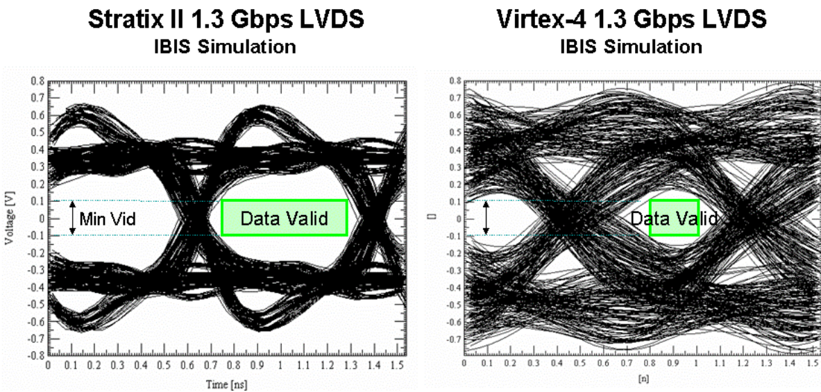
Figure 3: 1.3 Gbps LVDS IBIS simulation comparison of Stratix II and Virtex 4 eye-diagrams
