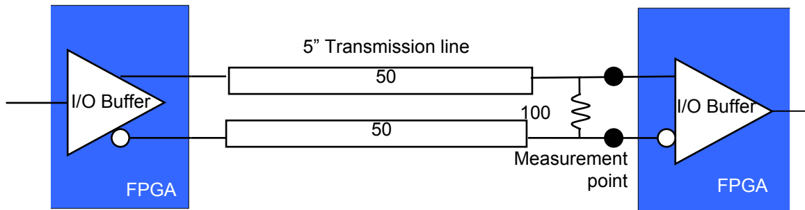
Figure 1: Simulation Setup for Measuring LVDS Eye Diagram for Stratix II and Virtex-4 FPGAs
