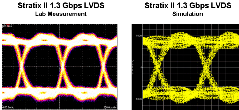
Figure 2: 1.3 Gbps LVDS comparison of Stratix II measured and simulation eye-diagrams
