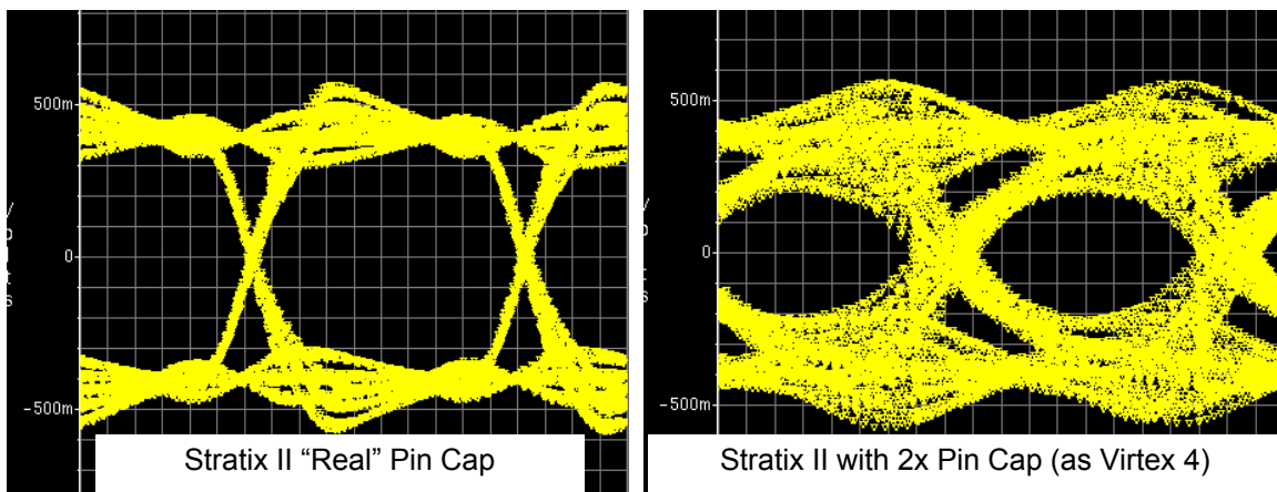
Figure 6: 1.0 Gbps LVDS IBIS Simulation Comparison of Stratix II with “Real” Pin Capacitance and Stratix II with 2X Pin Capacitance (as Virtex 4)
