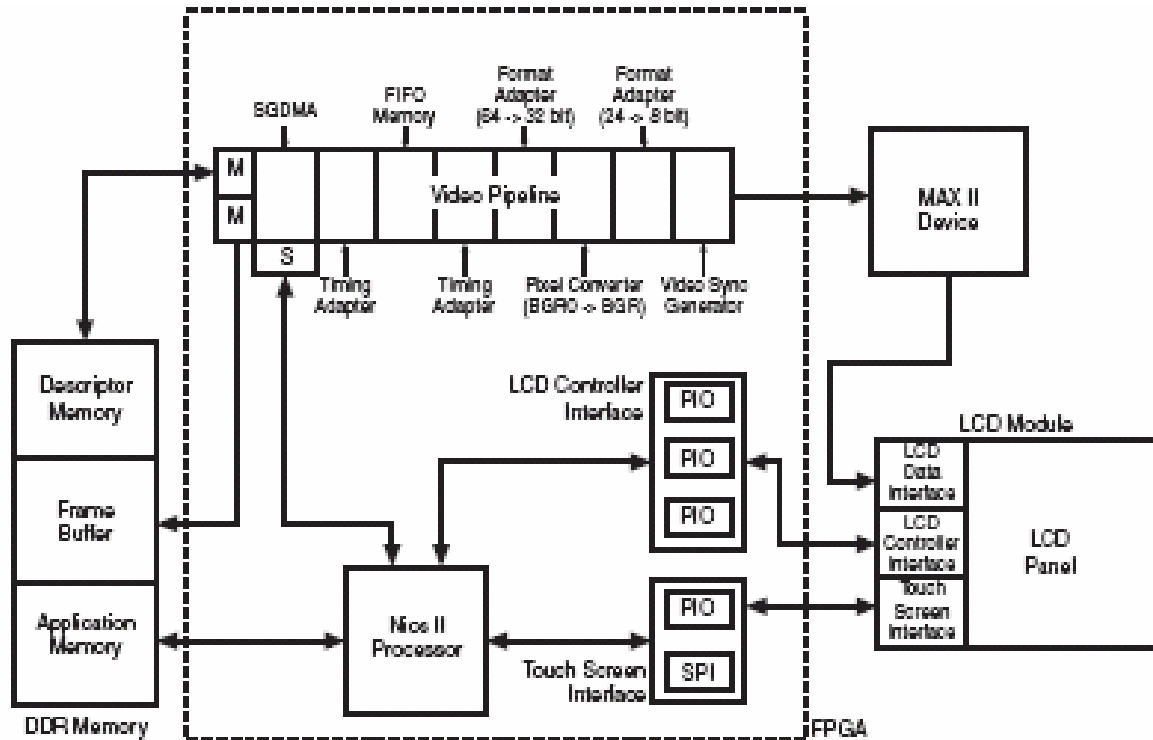
Figure 4. NEEK LCD Controller Subsystem
