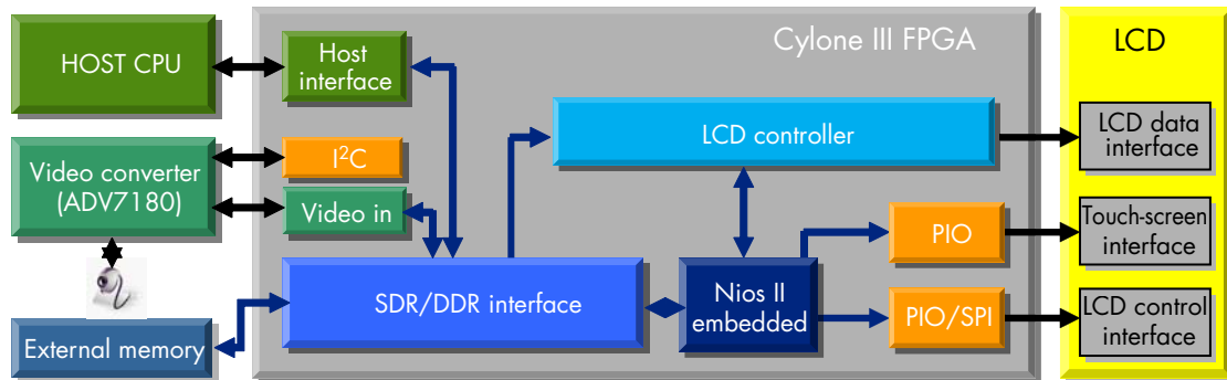
Figure 2. Touch-Screen Display Implementation With Cyclone III FPGA
