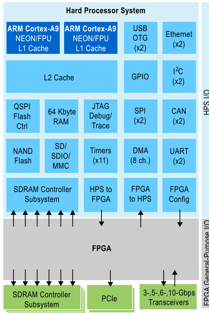
Figure 4. ARM-Based Hard Processor System Overview
