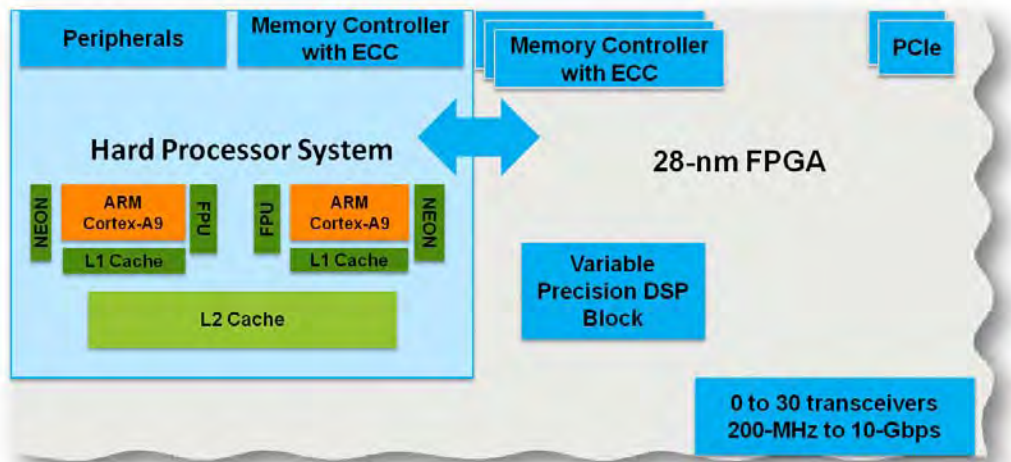
Figure 3. Processor Tightly Integrated with the FPGA Fabric
