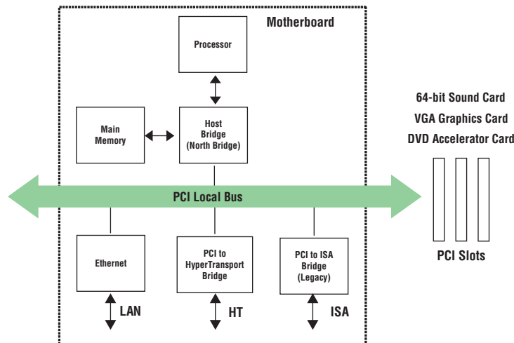
Figure 1. Typical PCI Local Bus System Application
