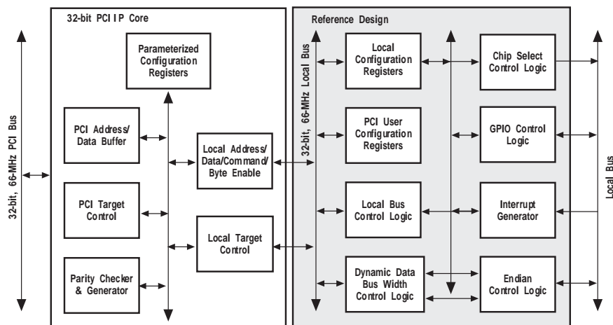
Figure 2. Altera’s MAX II CPLD-Based PCI Target Interface Solution Block Diagram
