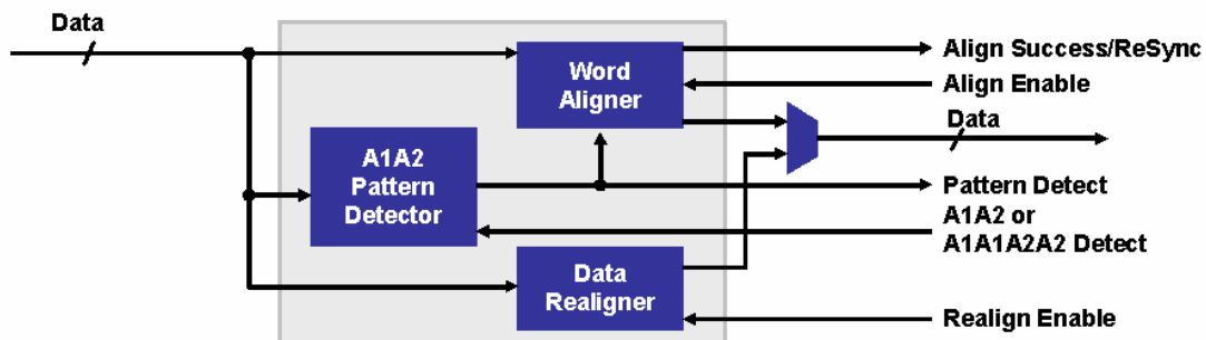
Figure 3. Block Diagram of a Pattern Detector for the Stratix GX Architecture
