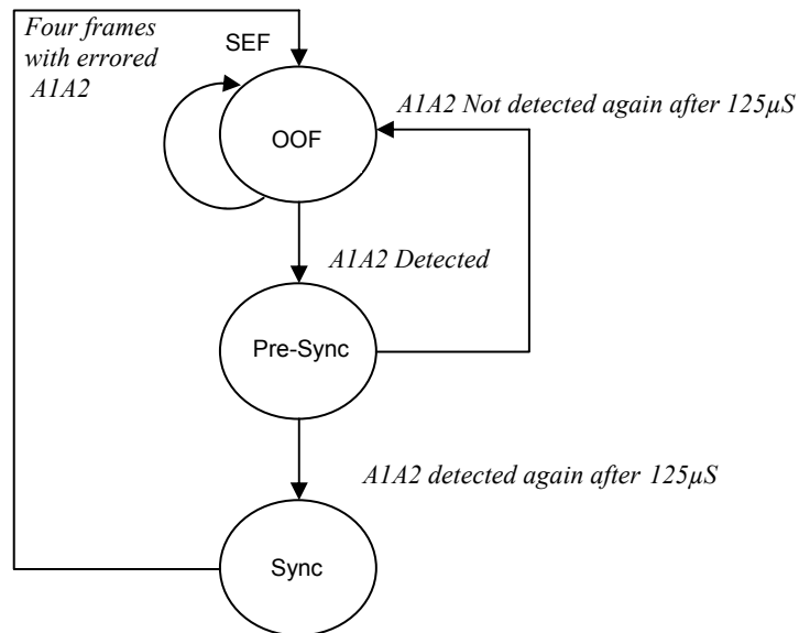
Figure 4 Finite State Machine to Confirm Frame Pattern
