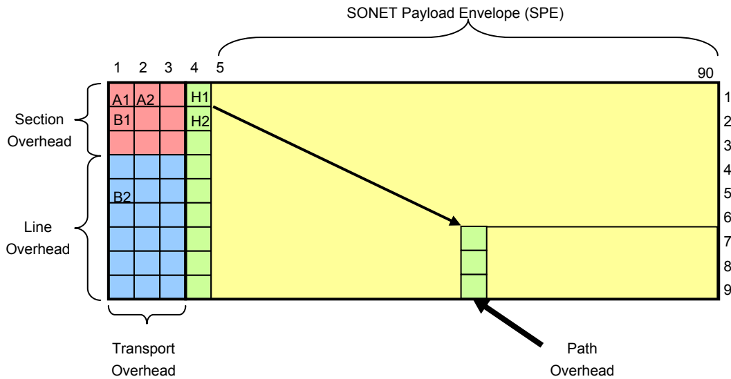
Figure 5 Typical SONET/SDH Frame for Backplane Application
