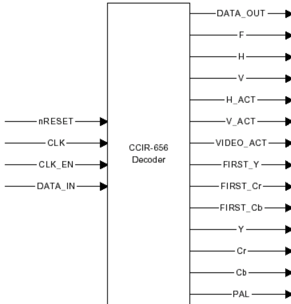
Figure 1. CCIR-656 Decoder Function
