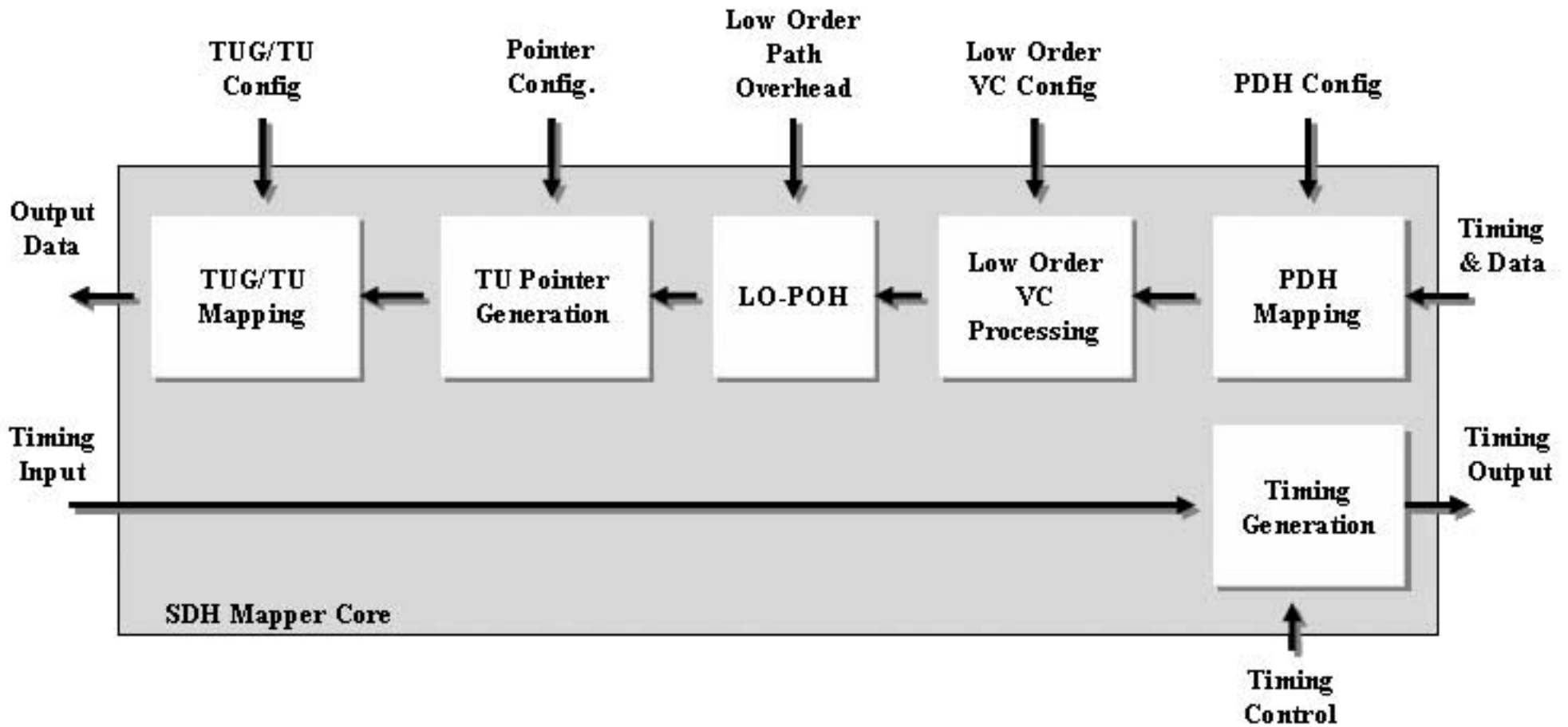
Figure 1. Mapper Block Diagram
