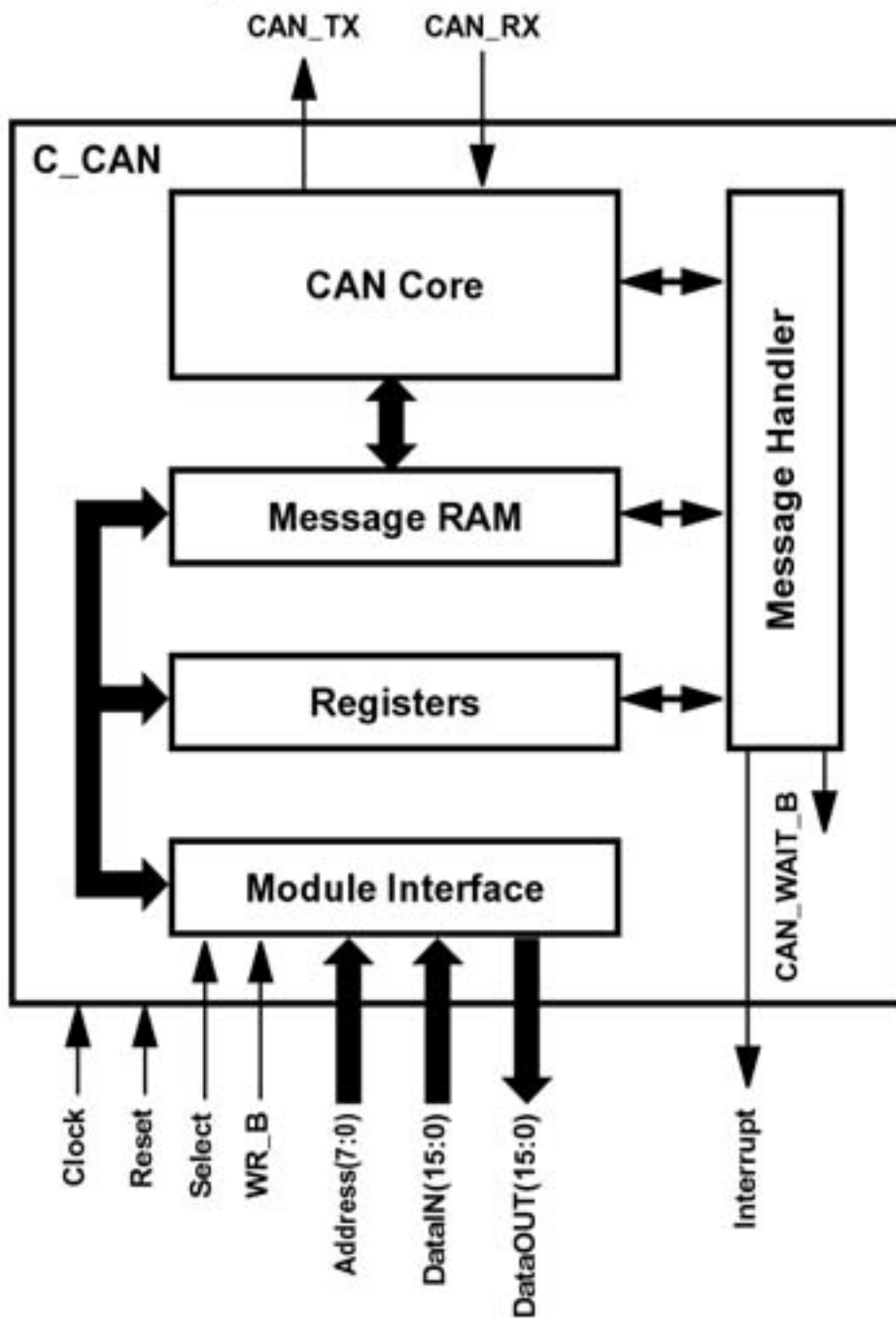
Figure 1. C_CAN Block Diagram
