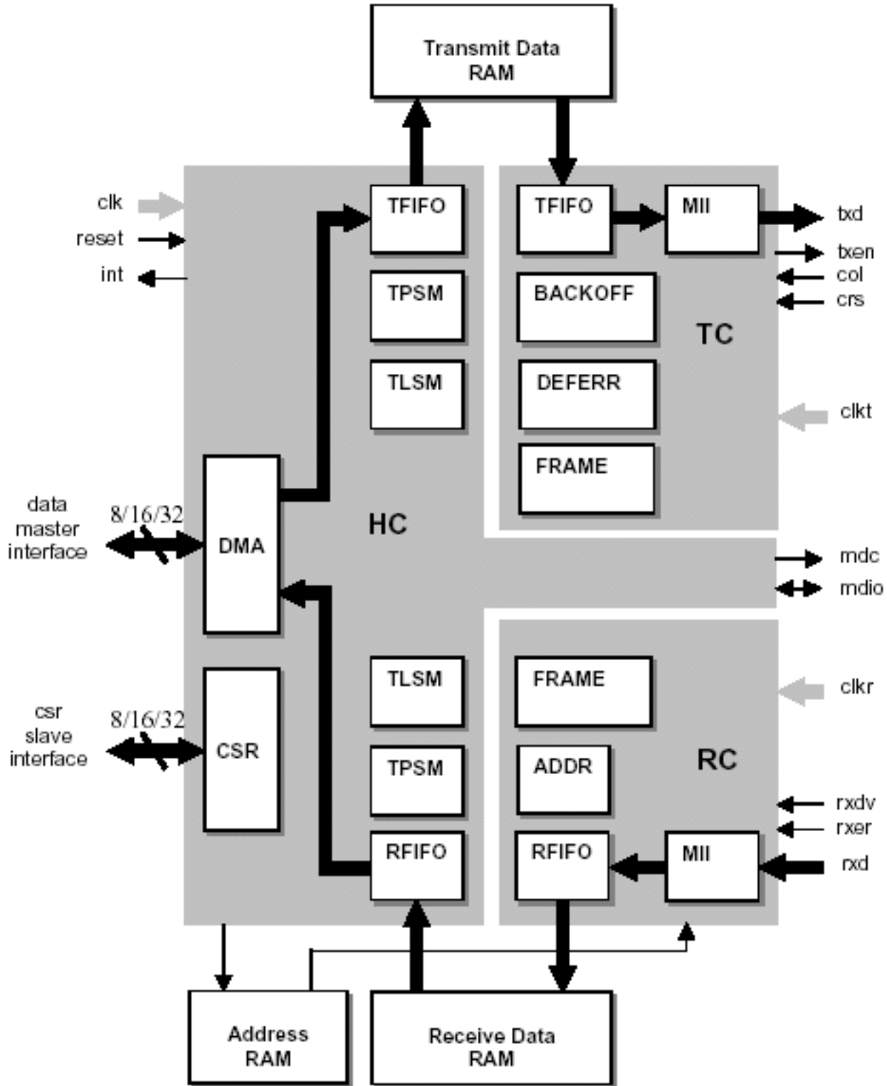
Figure 1. MAC Ethernet Controller Block Diagram
