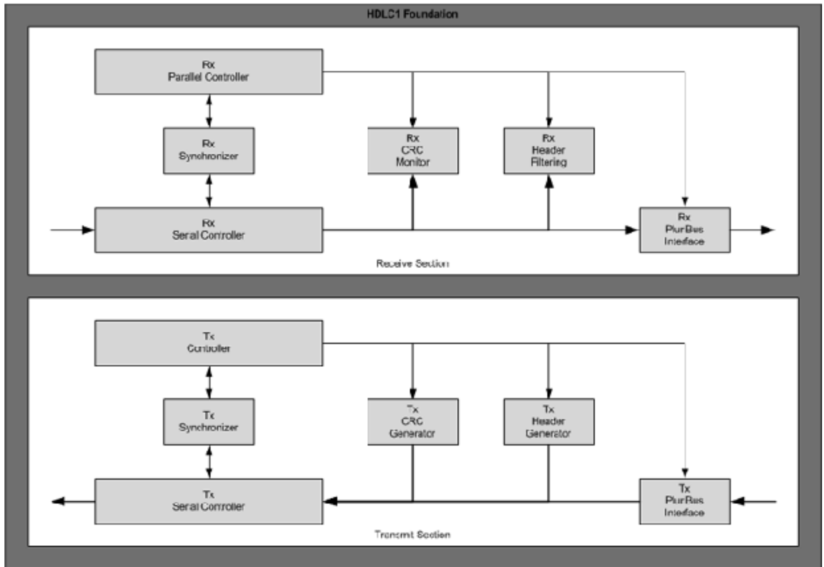
Figure 1. Block Diagram
