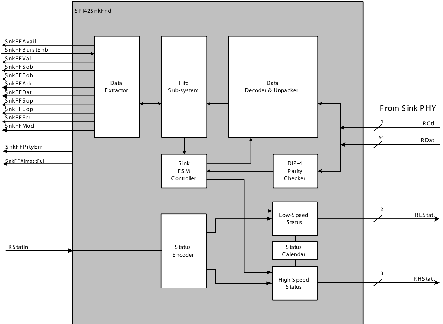
Figure 1. SPI4.2 Foundation Sink Block Diagram
