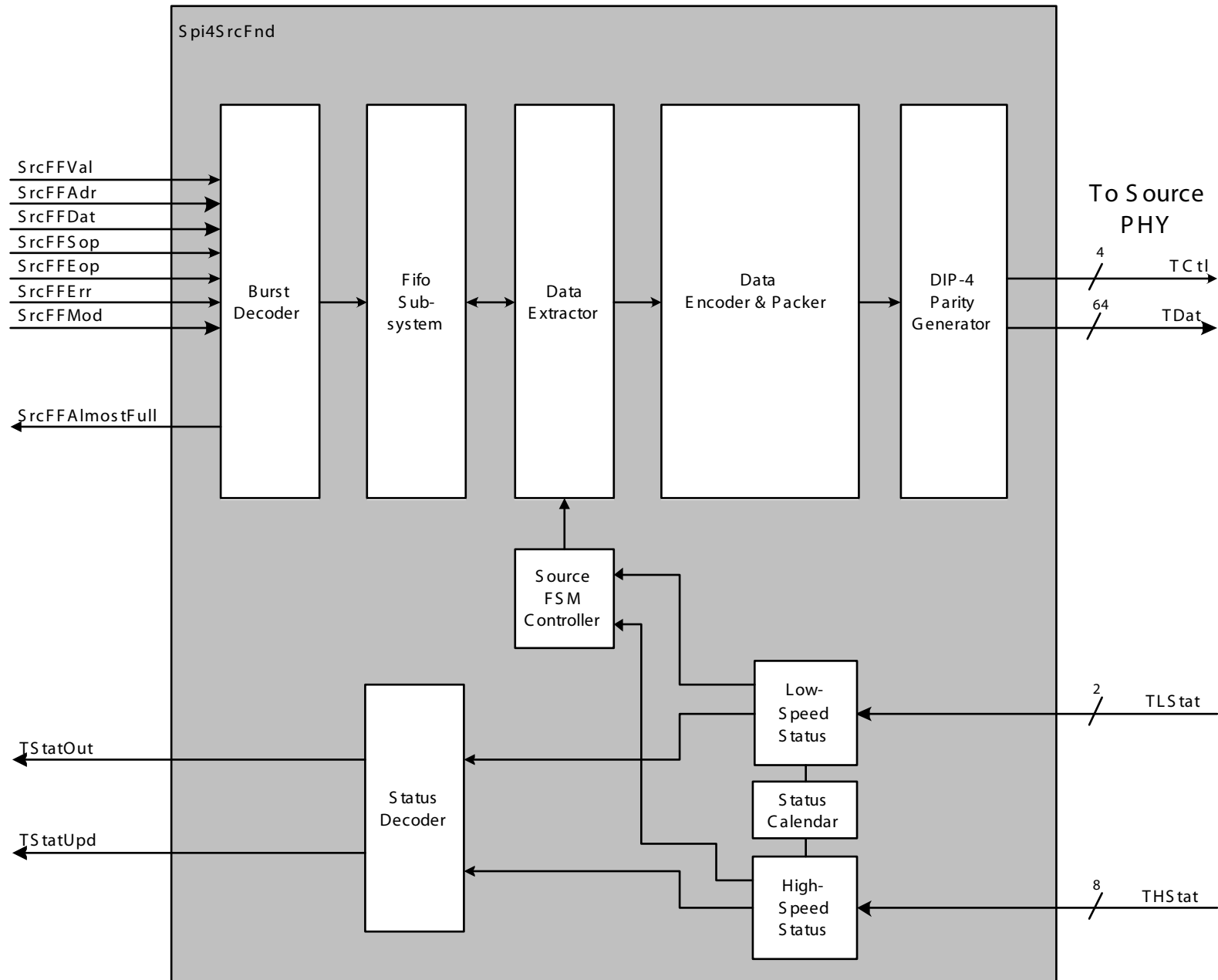
Figure 2. SPI4.2 Foundation Source Block Diagram
