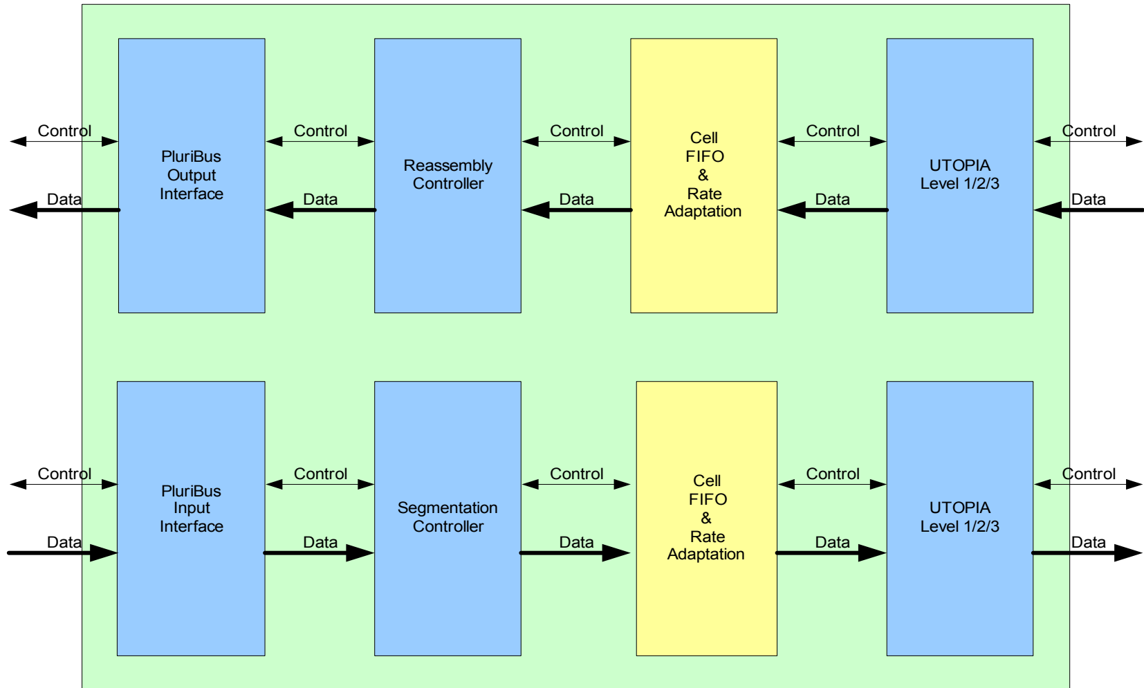
Figure 1. AA15 Block Diagram
