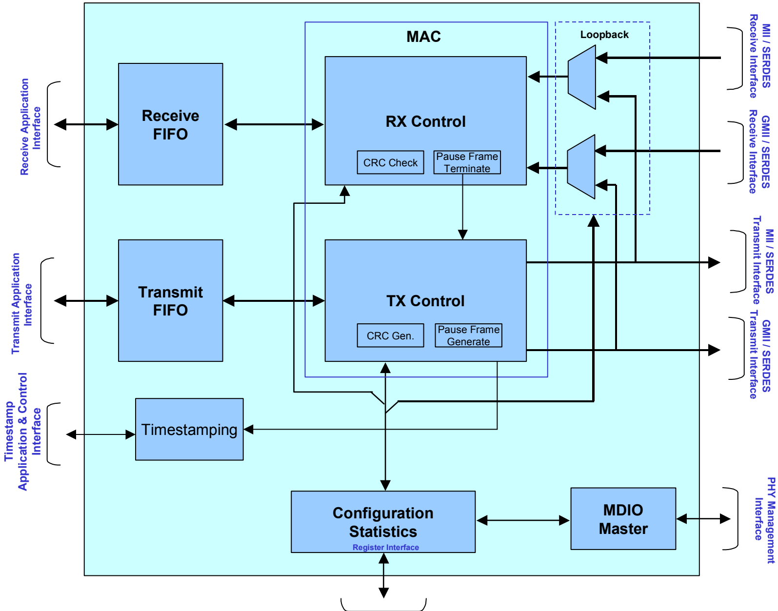
Figure 1. Tri-Speed 1588 Ethernet MAC Core
