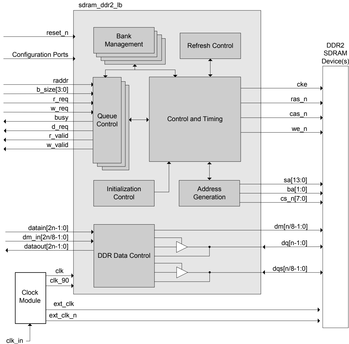
Figure 1. Northwest Logic DDR2 SDRAM Controller Block Diagram
