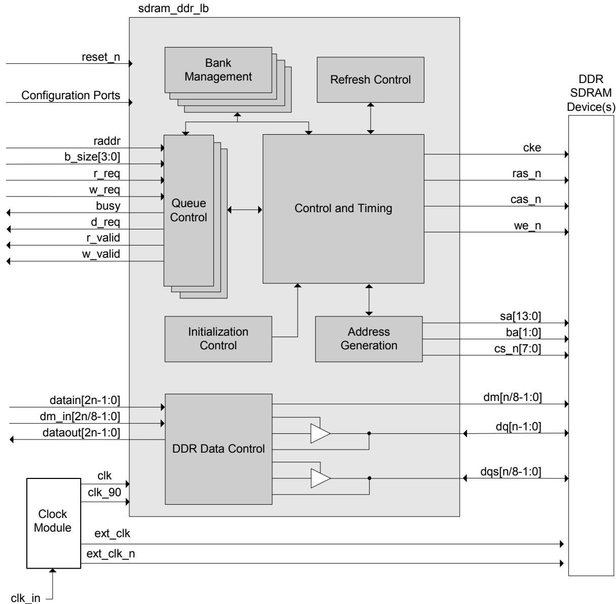
Figure 1. Block Diagram for Northwest Logic Mobile DDR SDRAM Controller Core
