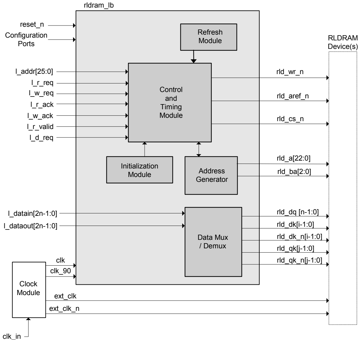
Figure 1. Block Diagram for the Megafunction
