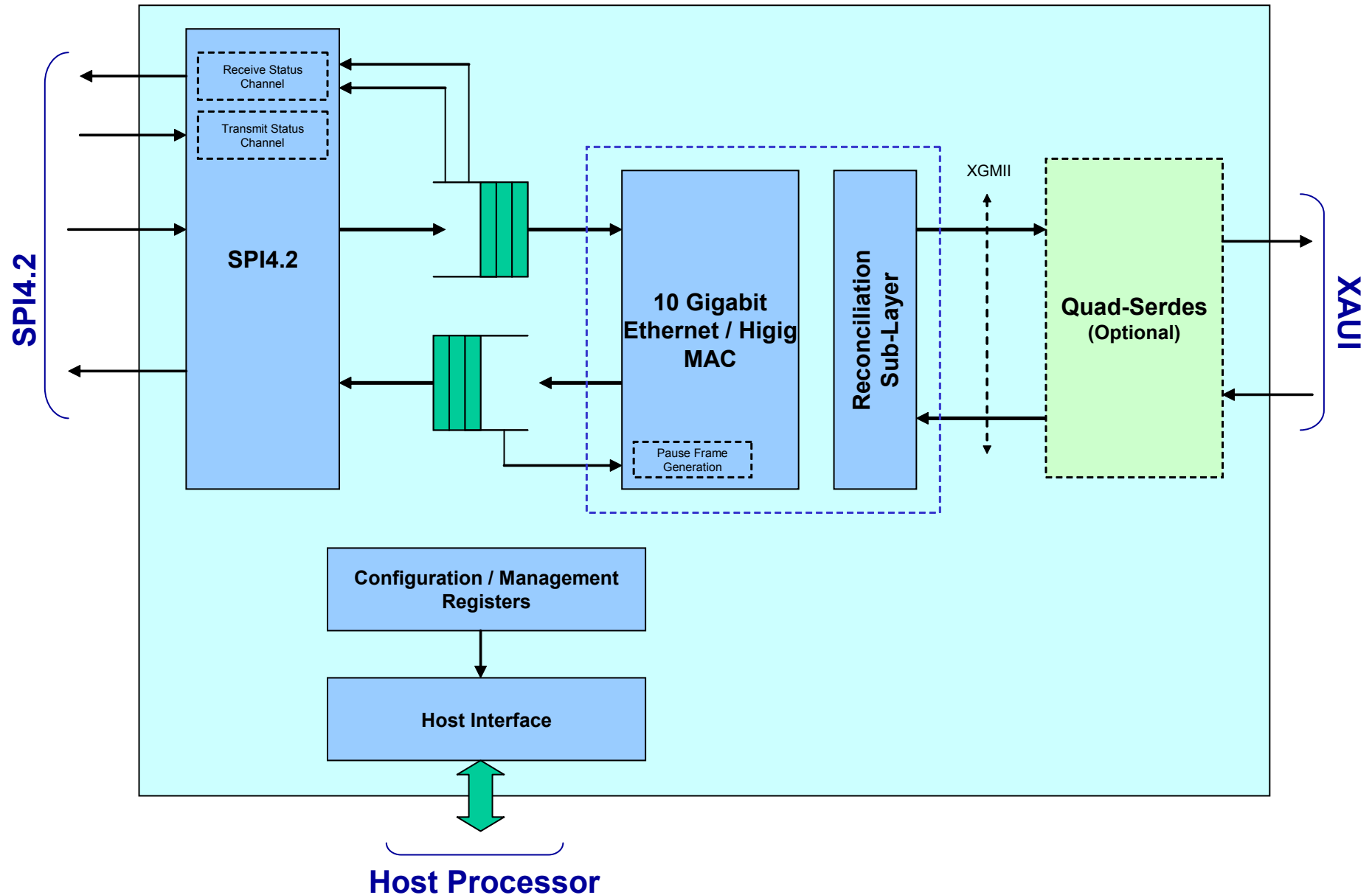
Figure 1. XS4 Bridge With Block Diagram
