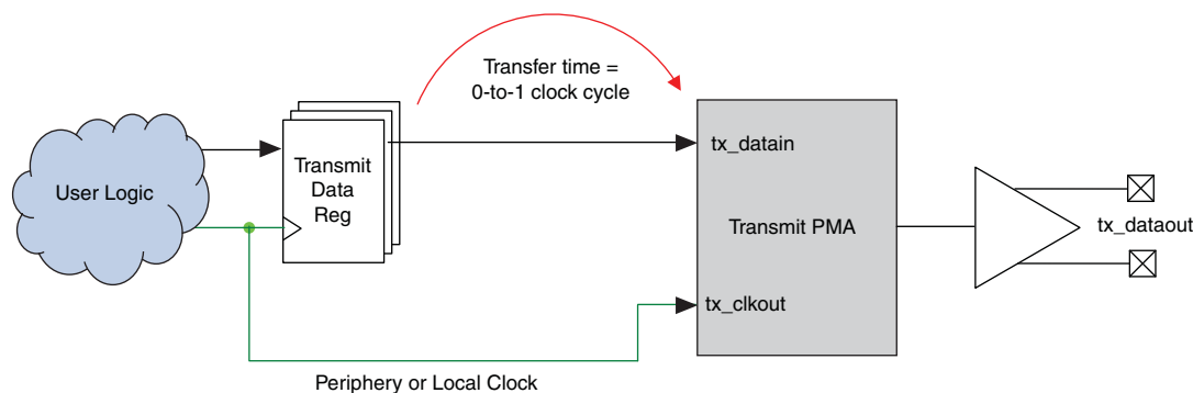
Figure 3. Single Channel Configured in Basic (PMA Direct) Functional Mode with a Positive Edge-Clocked Register
