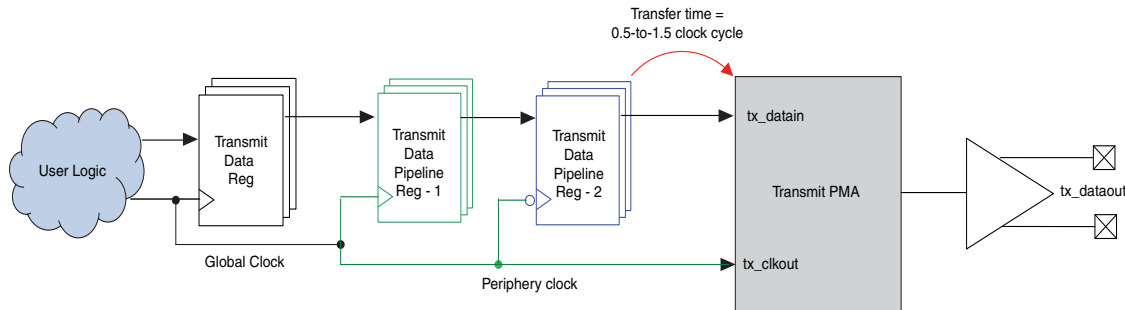
Figure 4. Negative Edge-Triggered Pipeline Registers to Meet the Timing Requirement at Higher Data Rates
