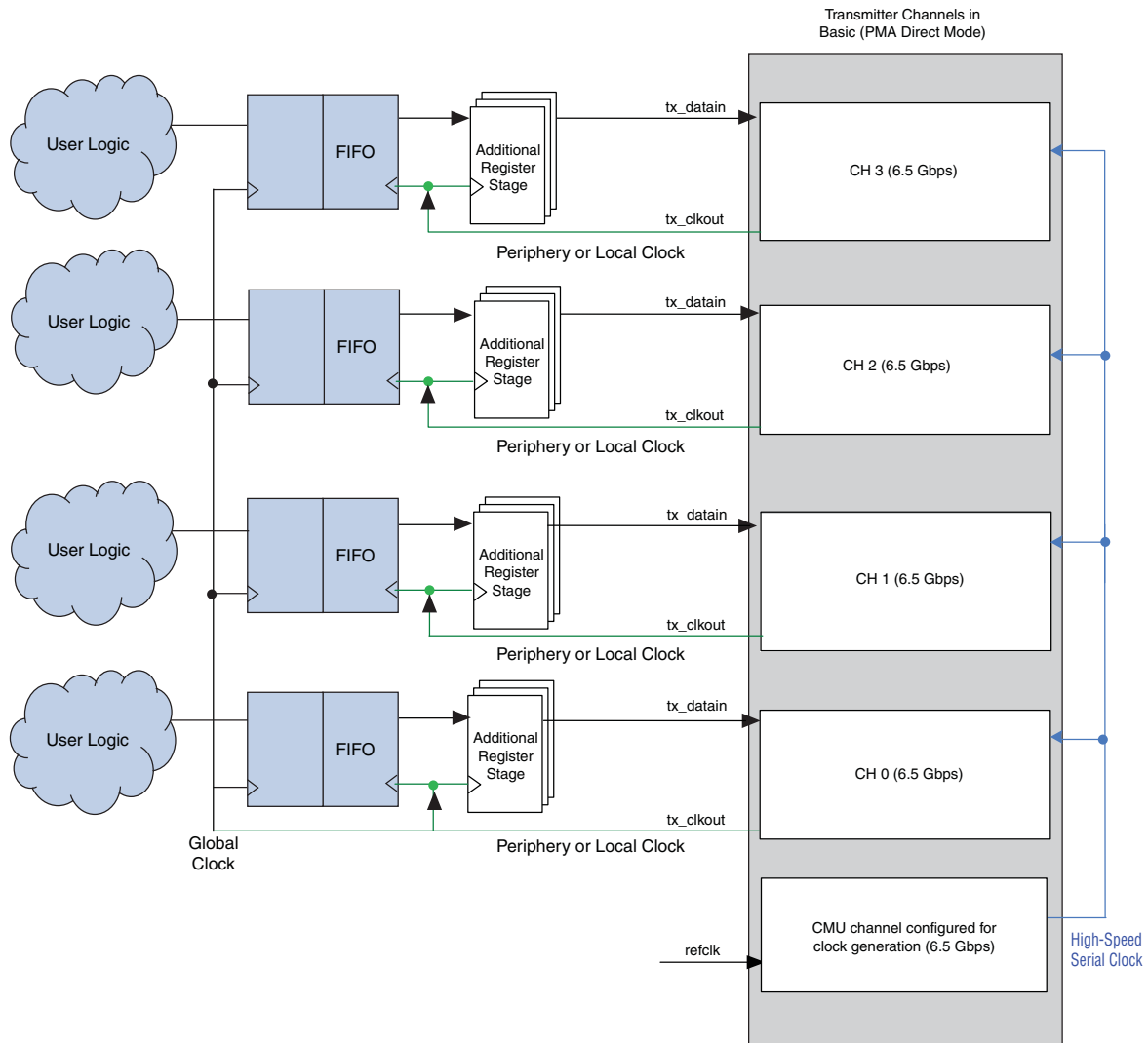
Figure 5. Multiple Channels Using FIFOs
