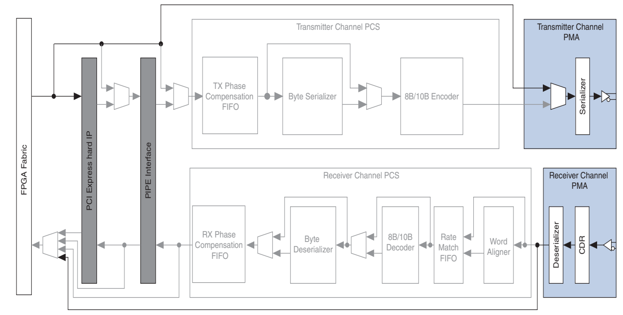
Figure 1. Basic (PMA Direct) Functional Mode
