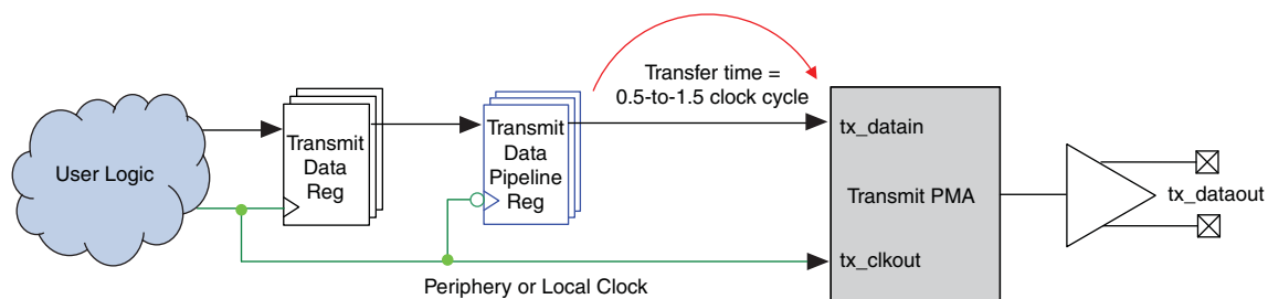
Figure 2. Negative Edge-Triggered Pipeline Registers to Meet the Timing Requirement
