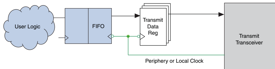
Figure 6. Transmit Transceiver with a Negative Edge-Clocked Register and a FIFO
