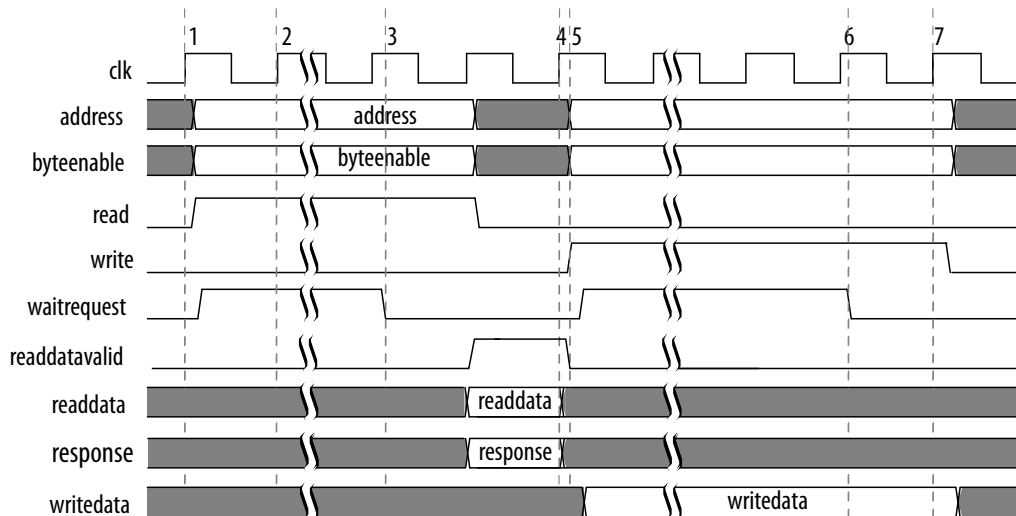
Figure 7. Read and Write Transfers with Waitrequest
