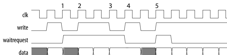
Figure 10. waitrequestAllowance Equals Two Transfers
