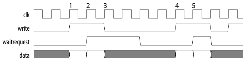
Figure 9. waitrequestAllowance Equals one Clock Cycle
