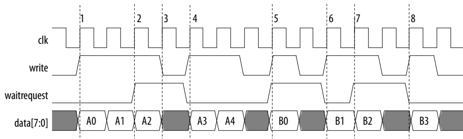
Figure 9. Master Write: waitrequestAllowance Equals one Clock Cycle
