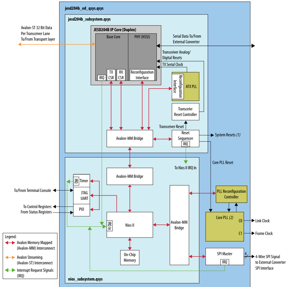
Figure 26. Qsys System
