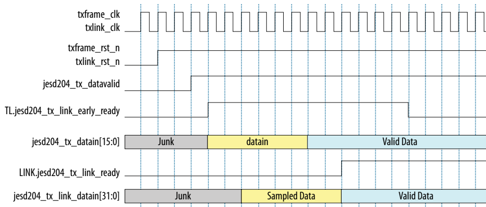
Figure 9. TX Data Transmission (For F = 8)
