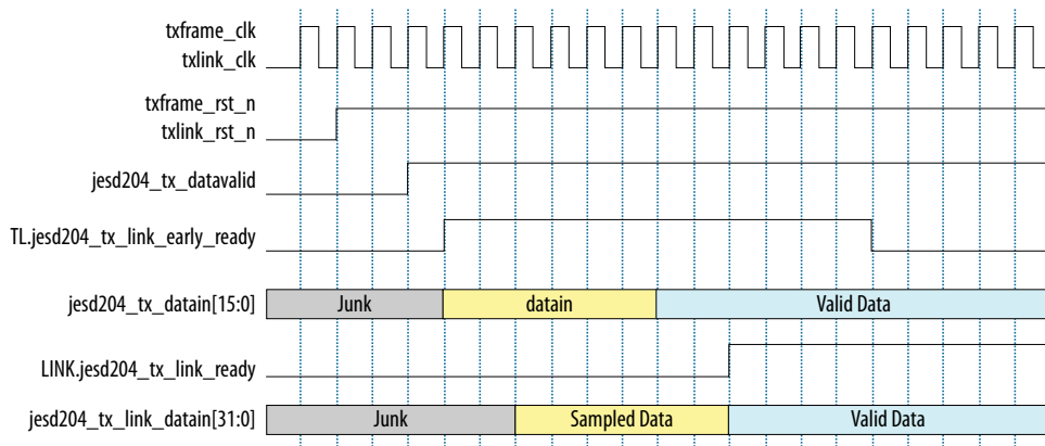
Figure 8. TX Data Transmission
