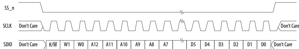
Figure 17. Serial Port Interface (24-bit) Timing Diagram
