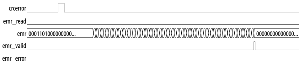
Figure 8. Example EMR Errors Timing Diagram
