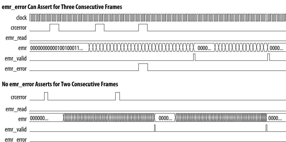
Figure 8. Example EMR Errors Timing Diagram
