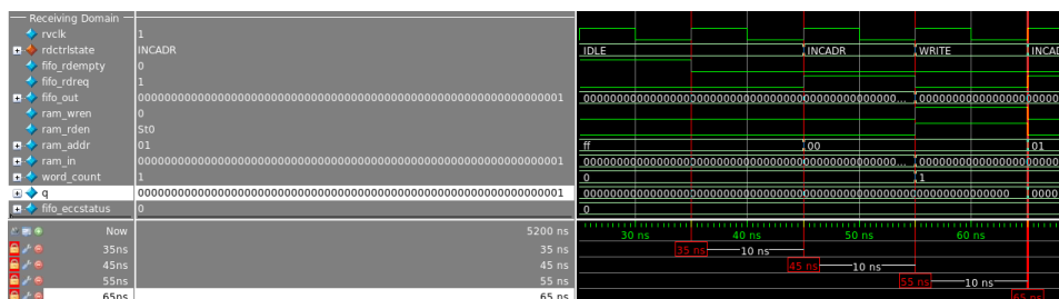
Figure 11. Initial Read Operation from the DCFIFO IP Core
