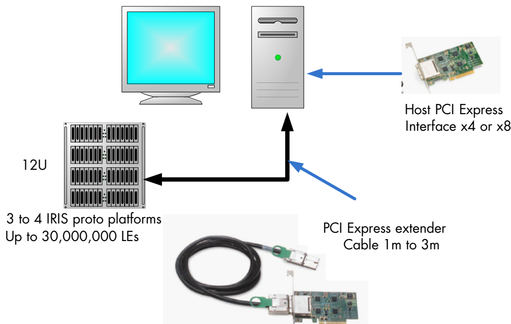
Figure 11. Scalable Rugged Prototyping, Simulation, and Emulation Platform
