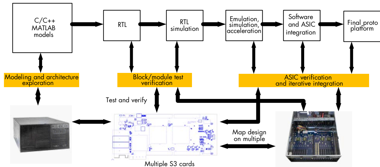
Figure 6. Typical ASIC Design Flow
