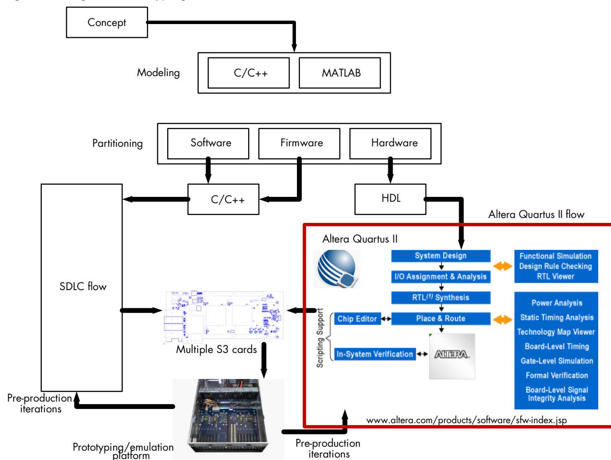
Figure 7. Integrated Prototyping and Emulation Flow
