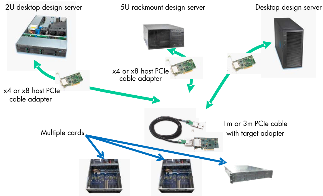
Figure 10. Enterprise-Level ASIC and Systems Prototyping, Simulation and Emulation Platform
