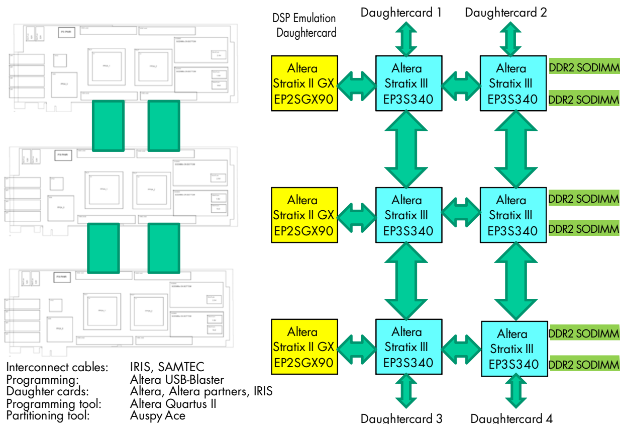
Figure 8. ASIC Prototyping and Emulation Stand-Alone Example 1
