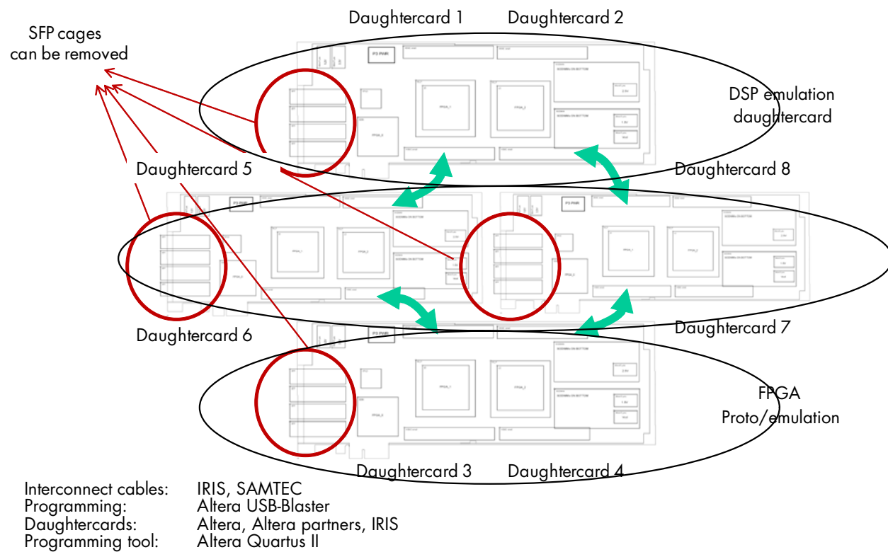
Figure 10. Enterprise-Level ASIC and Systems Prototyping, Simulation and Emulation Platform
