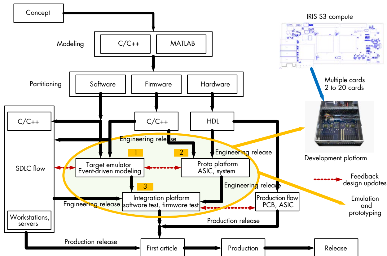
Figure 4. High-Level Integrated Product Design and Development Flow
