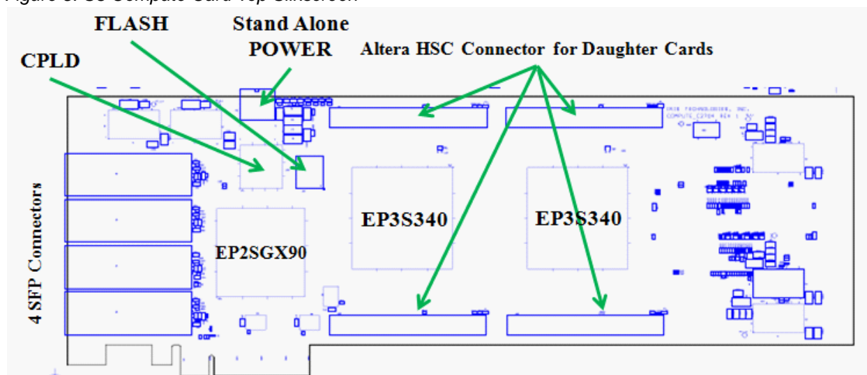
Figure 5. S3 Compute Card Top Silkscreen
