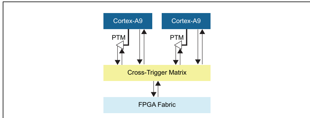
Figure 3. Cross-Triggering from the Software World to the Hardware World
