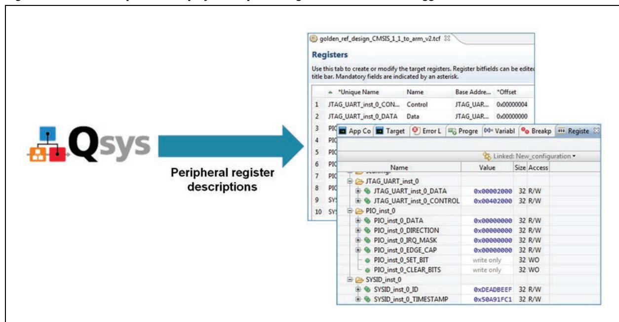
Figure 6. Automatic Import and Display of Peripheral Registers on the DS-5 Debugger
