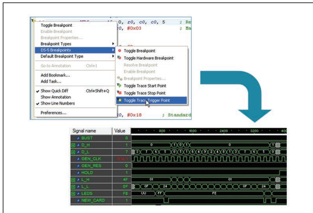
Figure 3. Cross-Triggering from the Software World to the Hardware World
