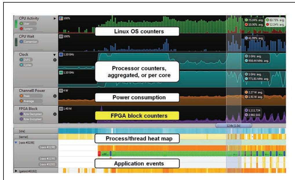
Figure 7. Timeline View in ARM DS-5 Streamline
