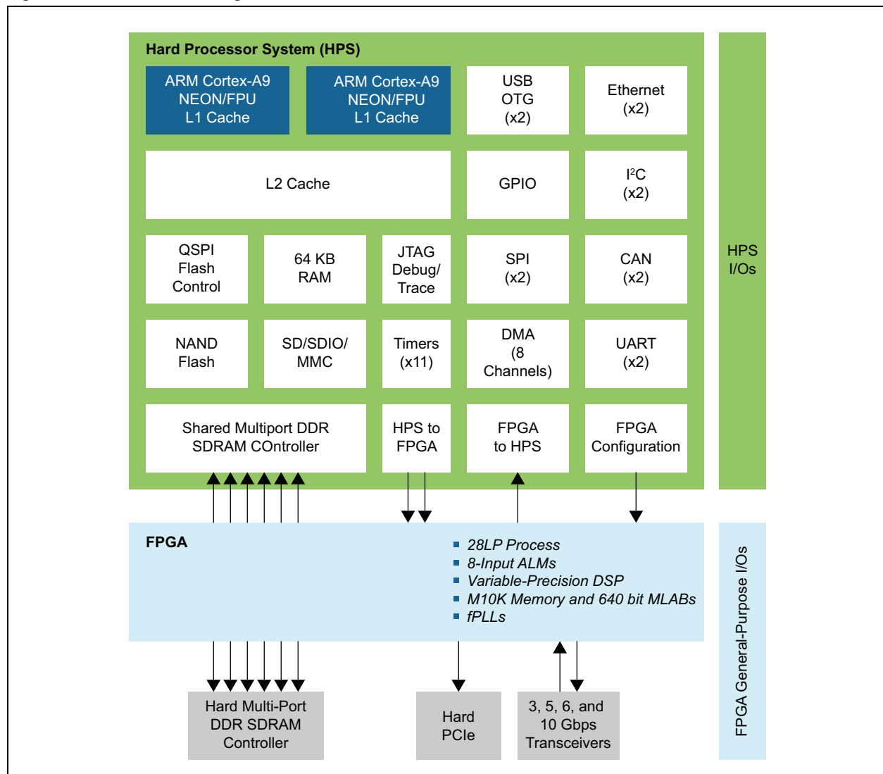
Figure 1. Altera SoC Block Diagram
